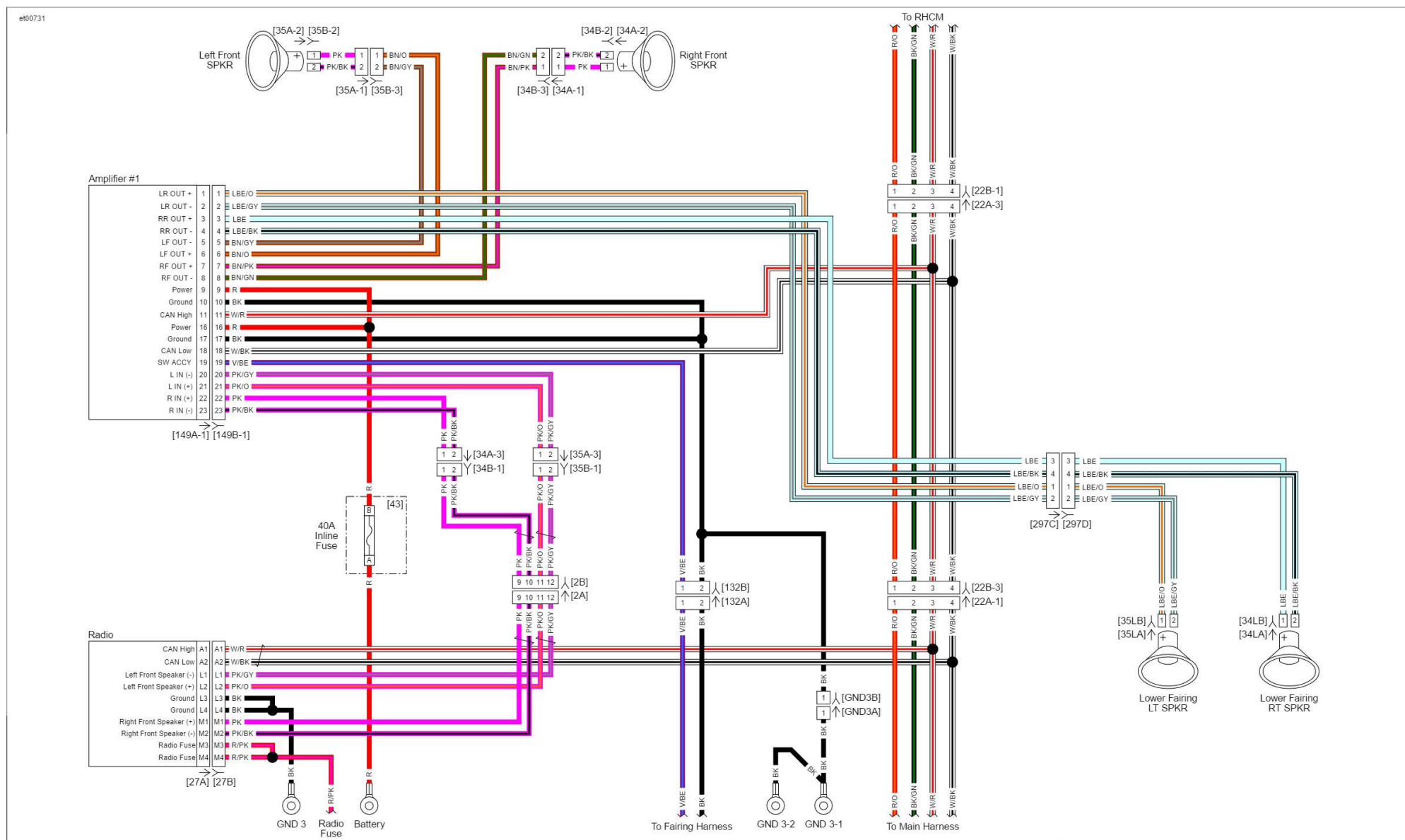
P&amp;A Radio with 2 Amps (1 of 2): 2016 Touring
