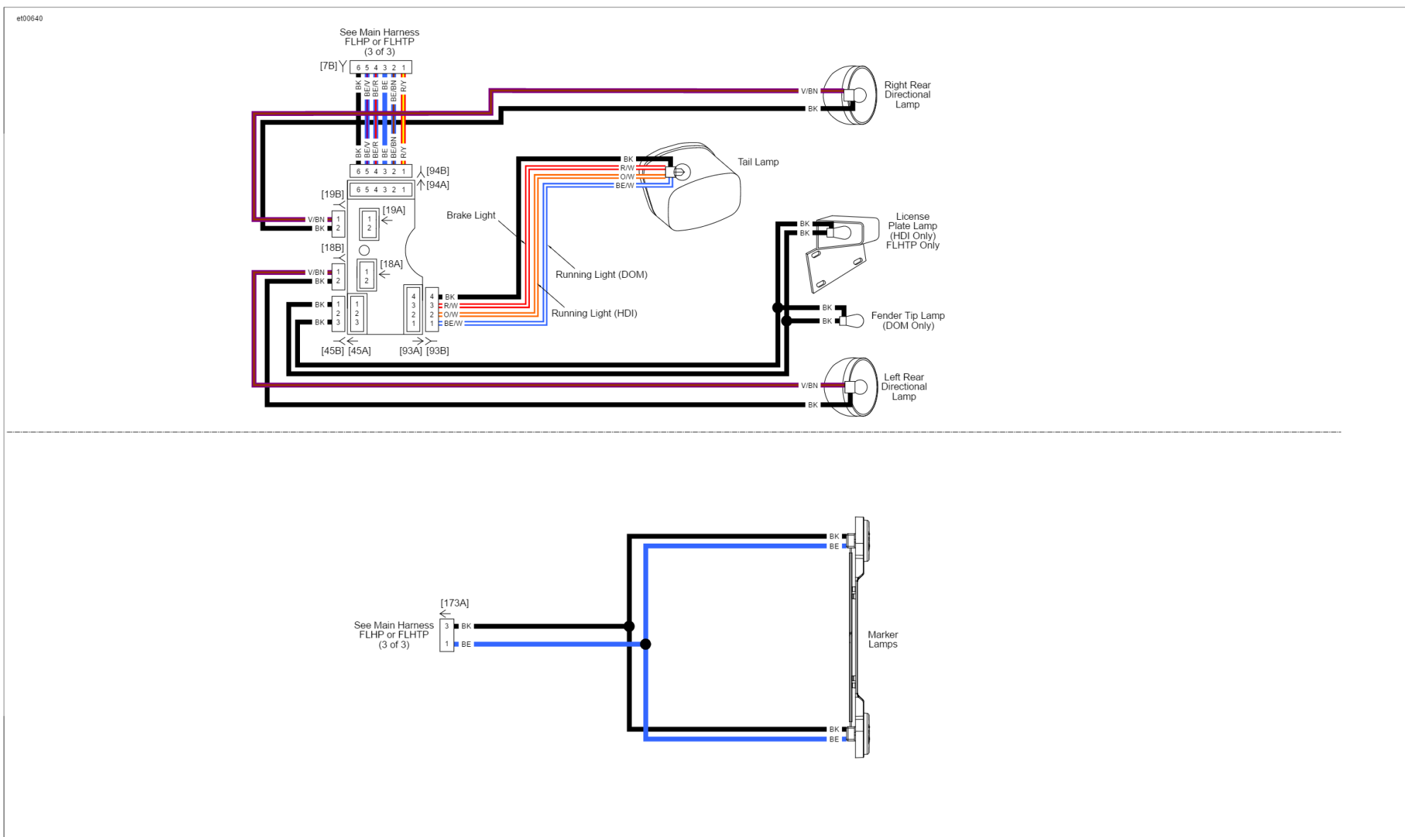
Rear Lighting: 2016 Police
