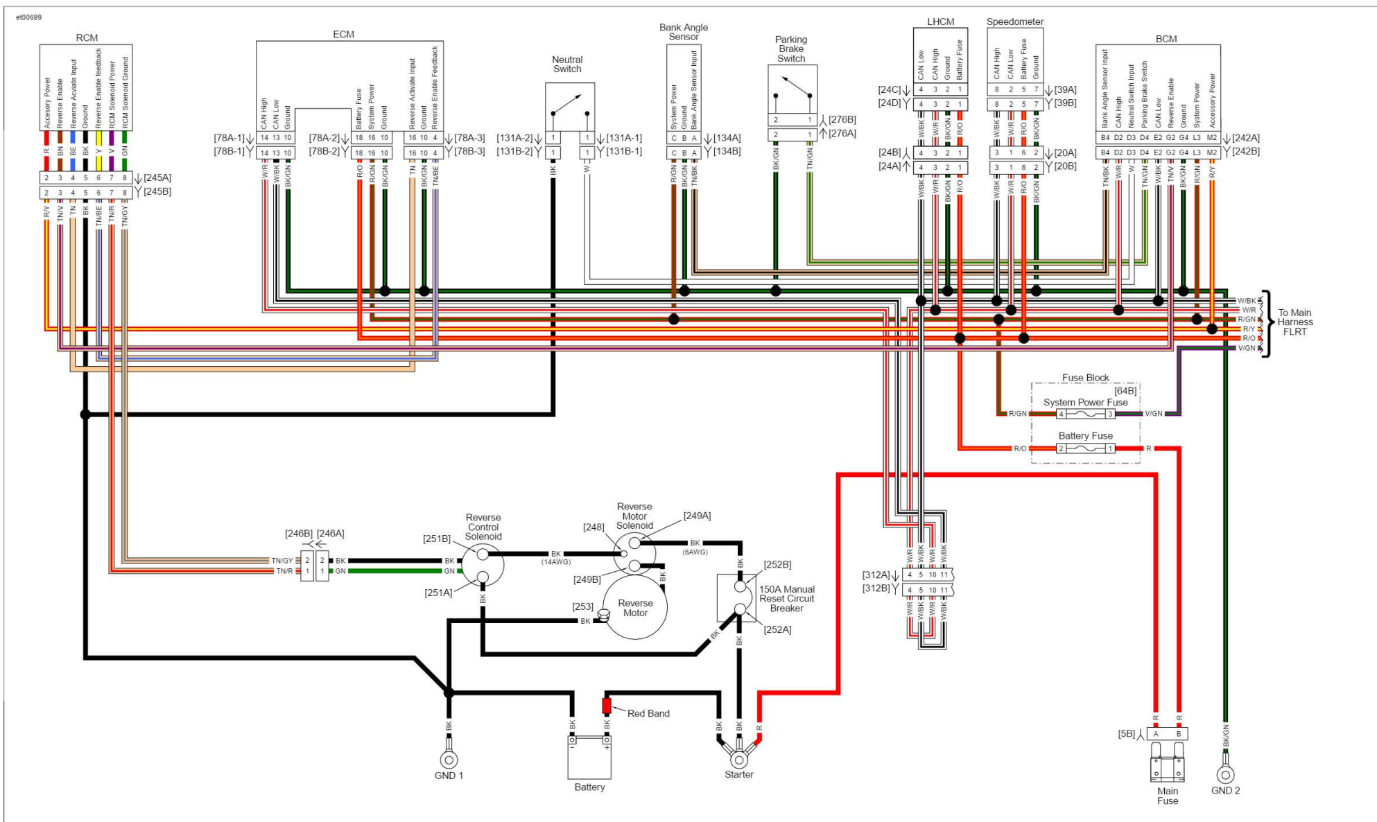
Reverse FLRT: 2016 Trike Model
