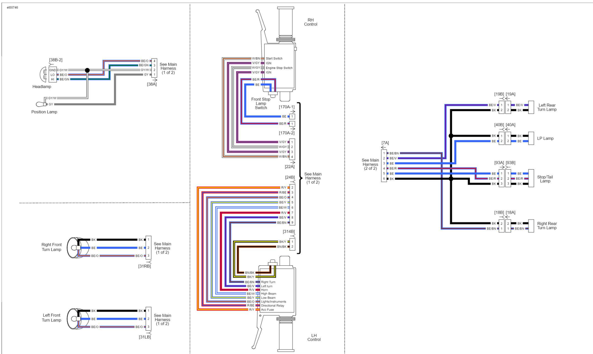
Lighting and Hand Controls: 2016 Street
