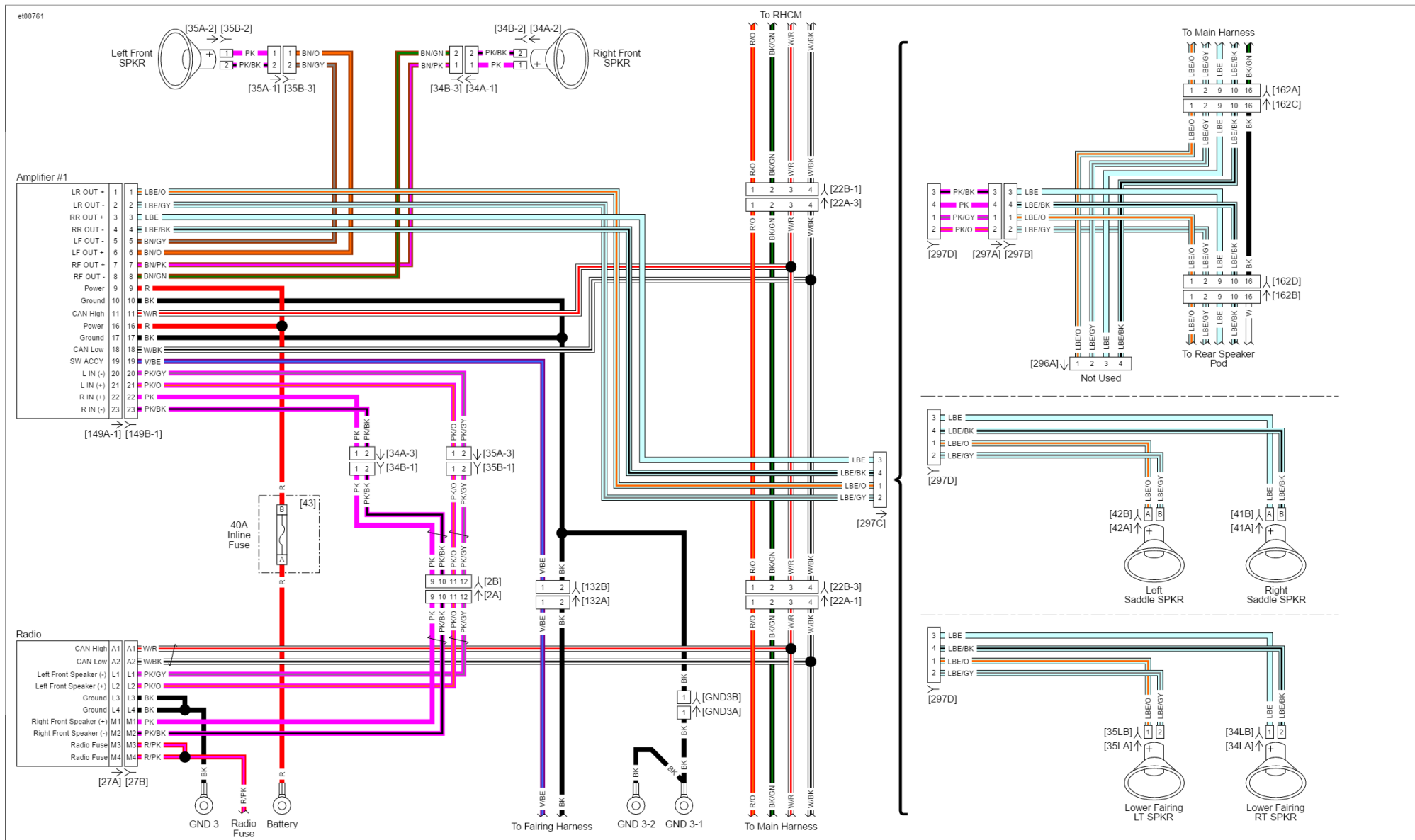
P&amp;A Radio with 1 Amp: 2016 Touring
