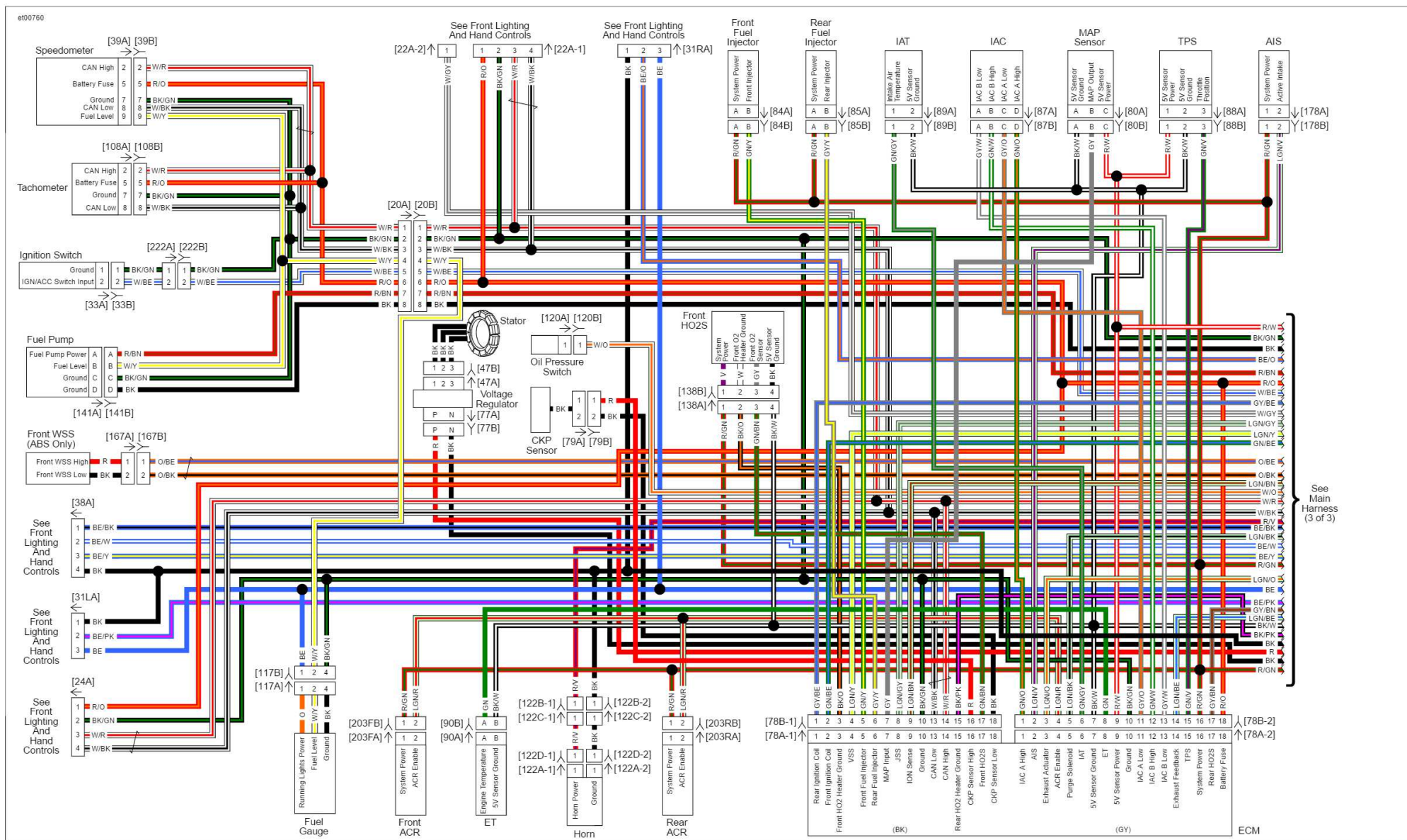
Main Harness 2 of 3 (FXDL): 2016 Dyna
