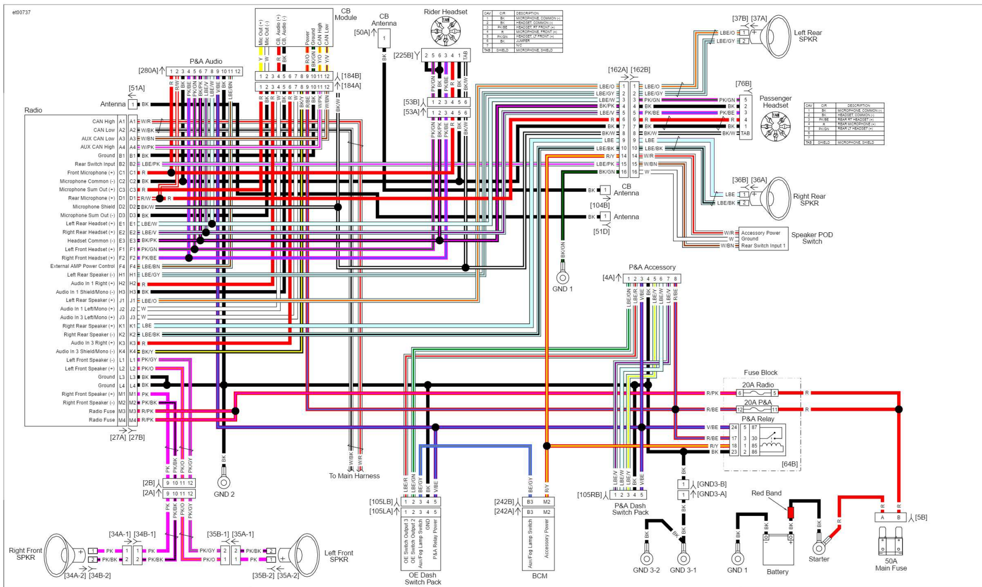
OE Radio: 2016 Touring (Except FLHX/S, FLT)
