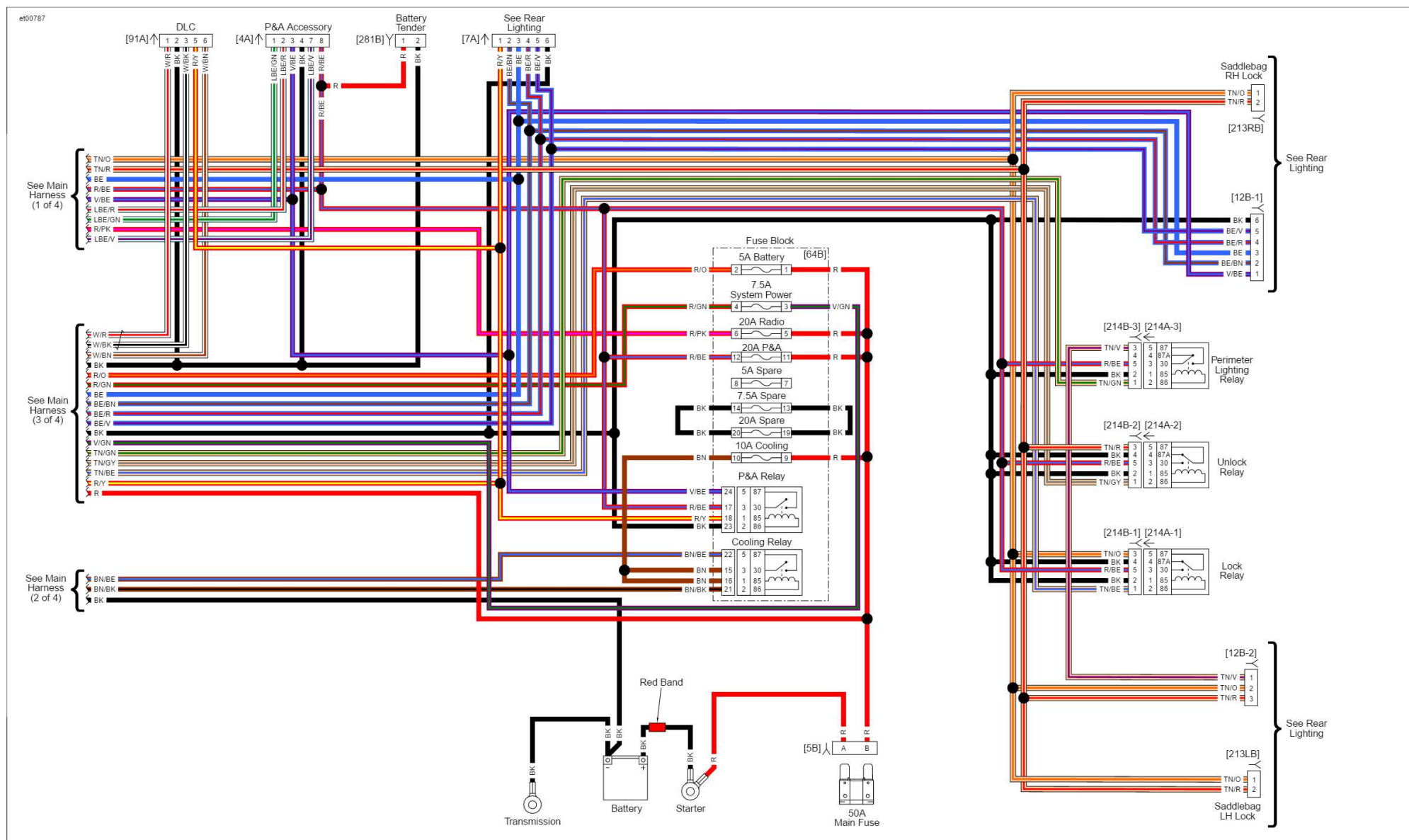
Main Harness (4 of 4): 2016 FLTRUSE
