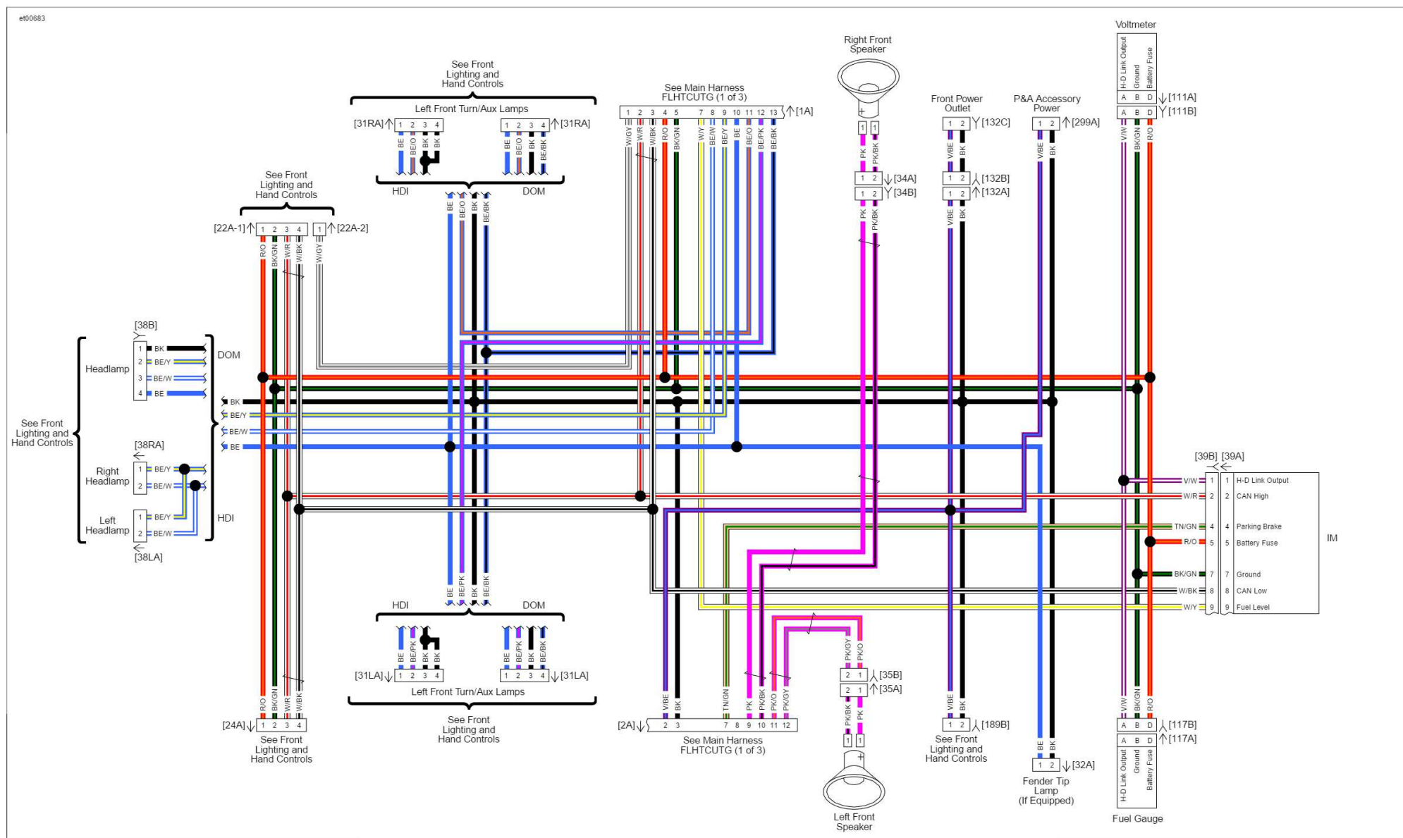
Fairing Harness FLHTCUTG: 2016 Trike Model
