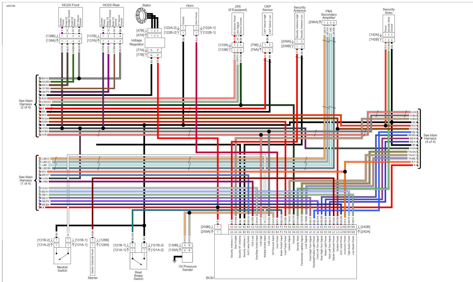
Main Harness (3 of 4): 2016 FLTRUSE
