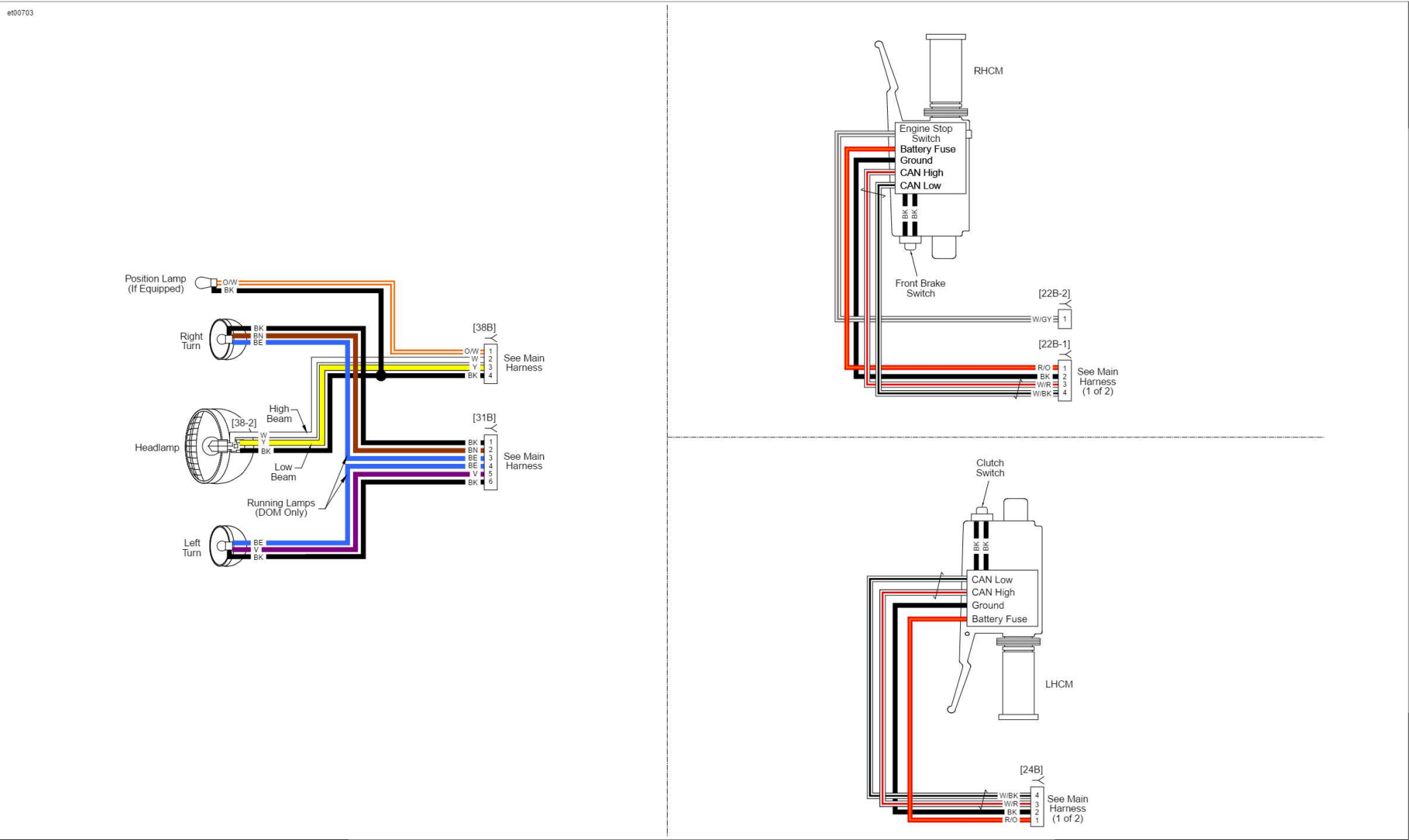
Front Lighting and Hand Controls: 2016 Sportster
