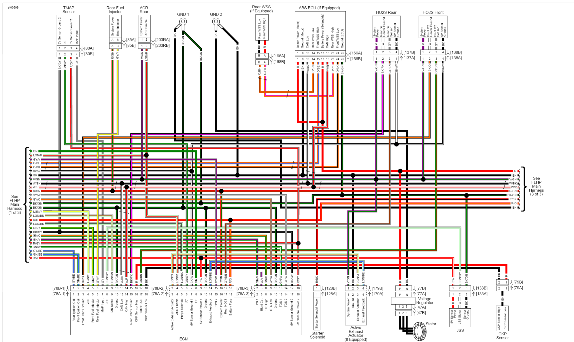
Main Harness (2 of 3): 2016 FLHP
