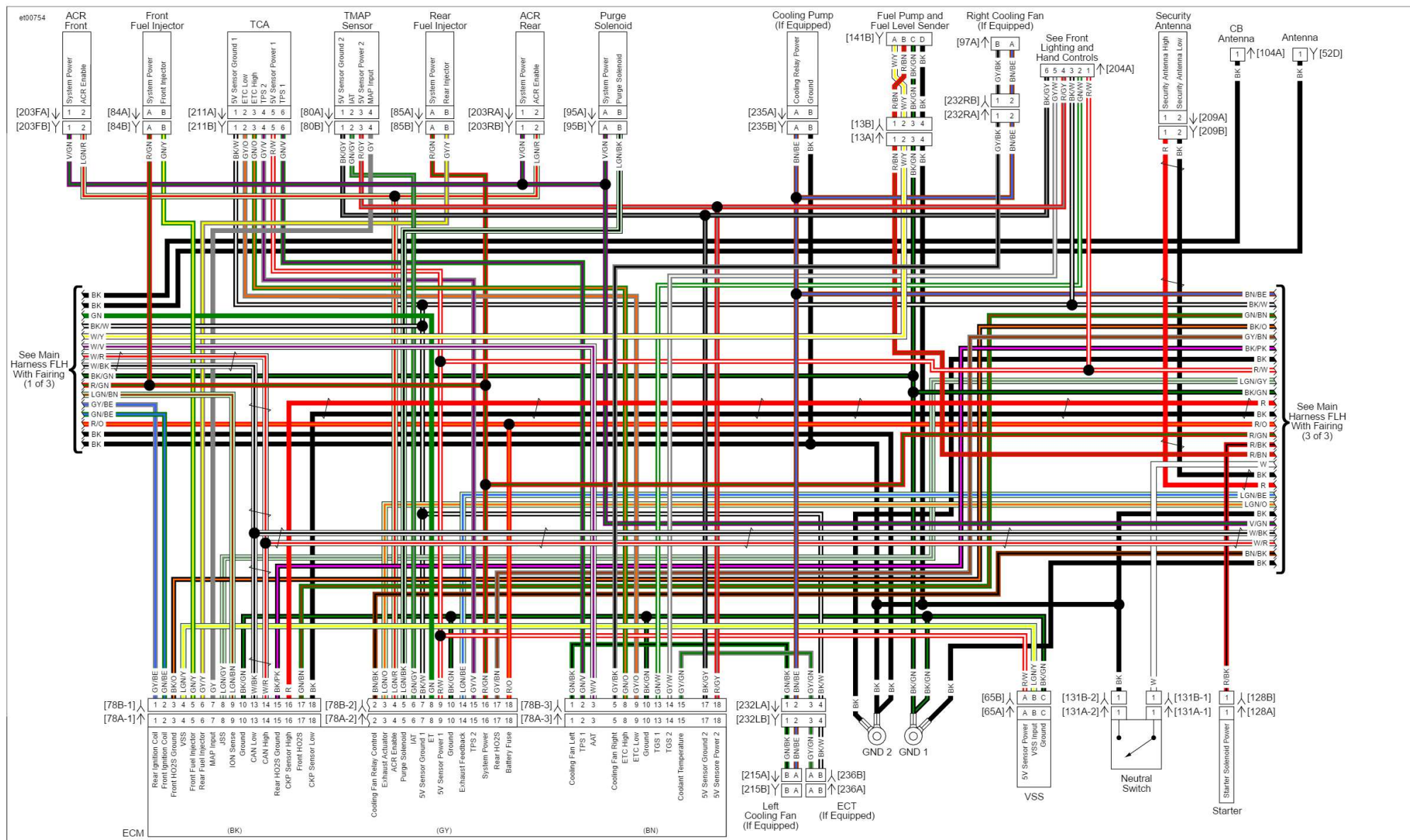
Main Harness FLH (2 of 3): 2016 Touring (with Fairing)
