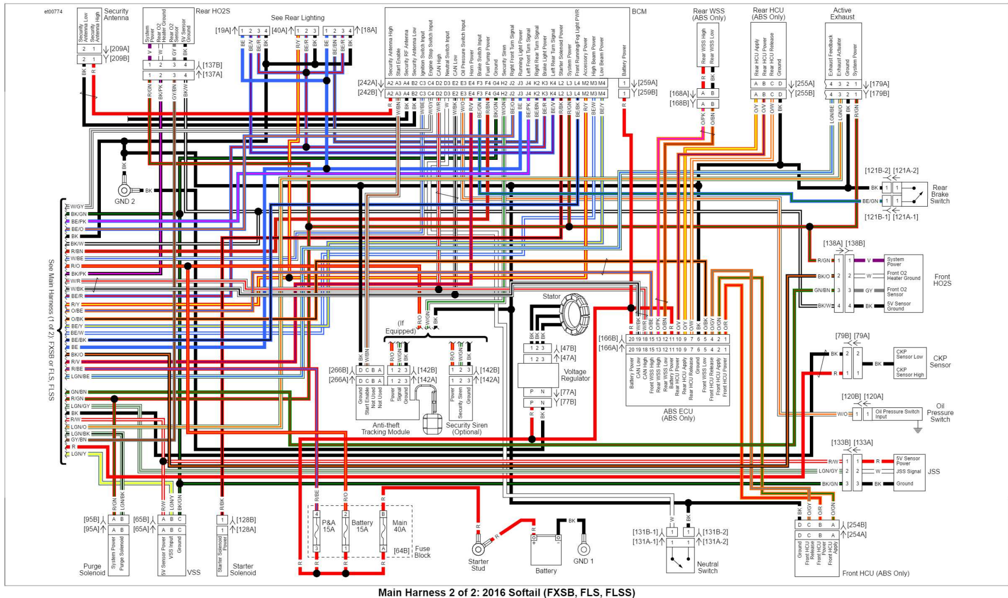
Main Harness 2 of 2: 2016 Softail (FXSB, FLS, FLSS)
