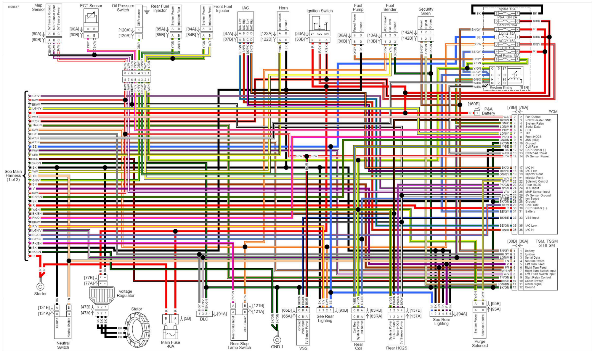
Main Harness (2 of 2): 2016 V-Rod
