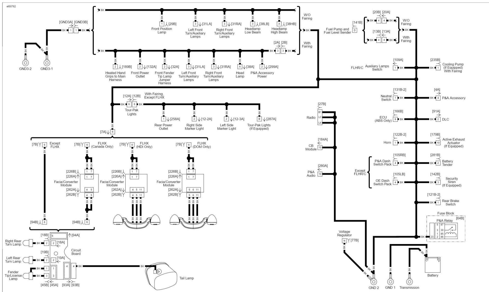
Ground Circuit FLH: 2016 Touring
