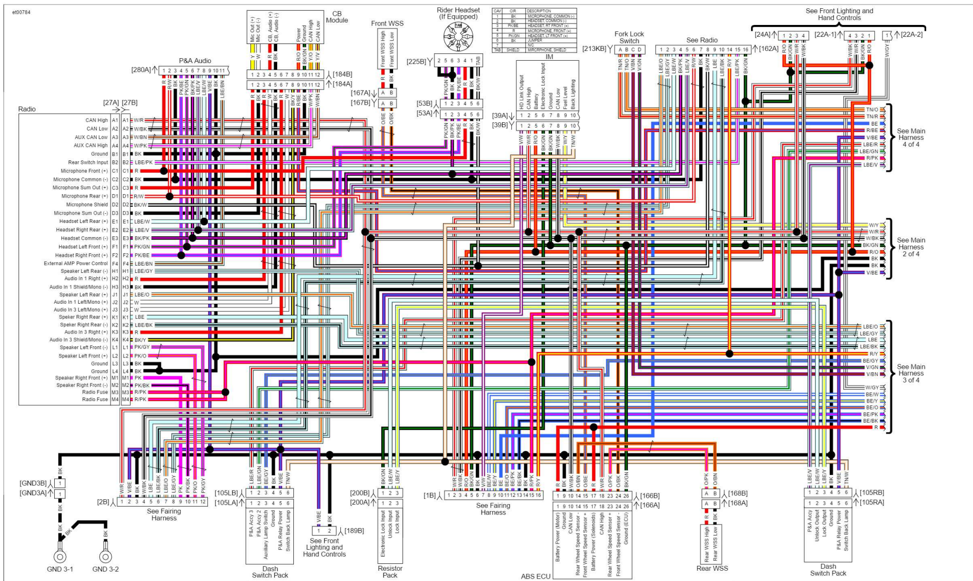
Main Harness (1 of 4): 2016 FLTRUSE
