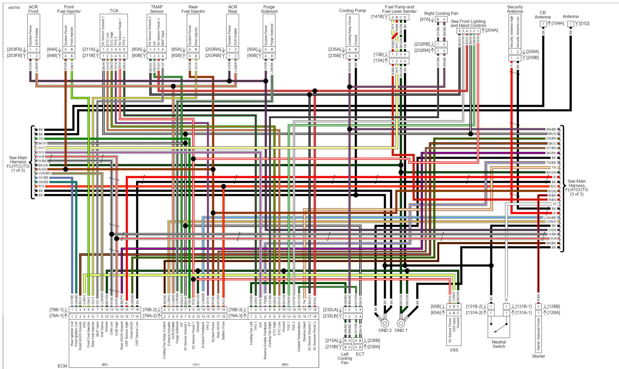
Main Harness FLHTCUTG (2 of 3): 2016 Trike Model
