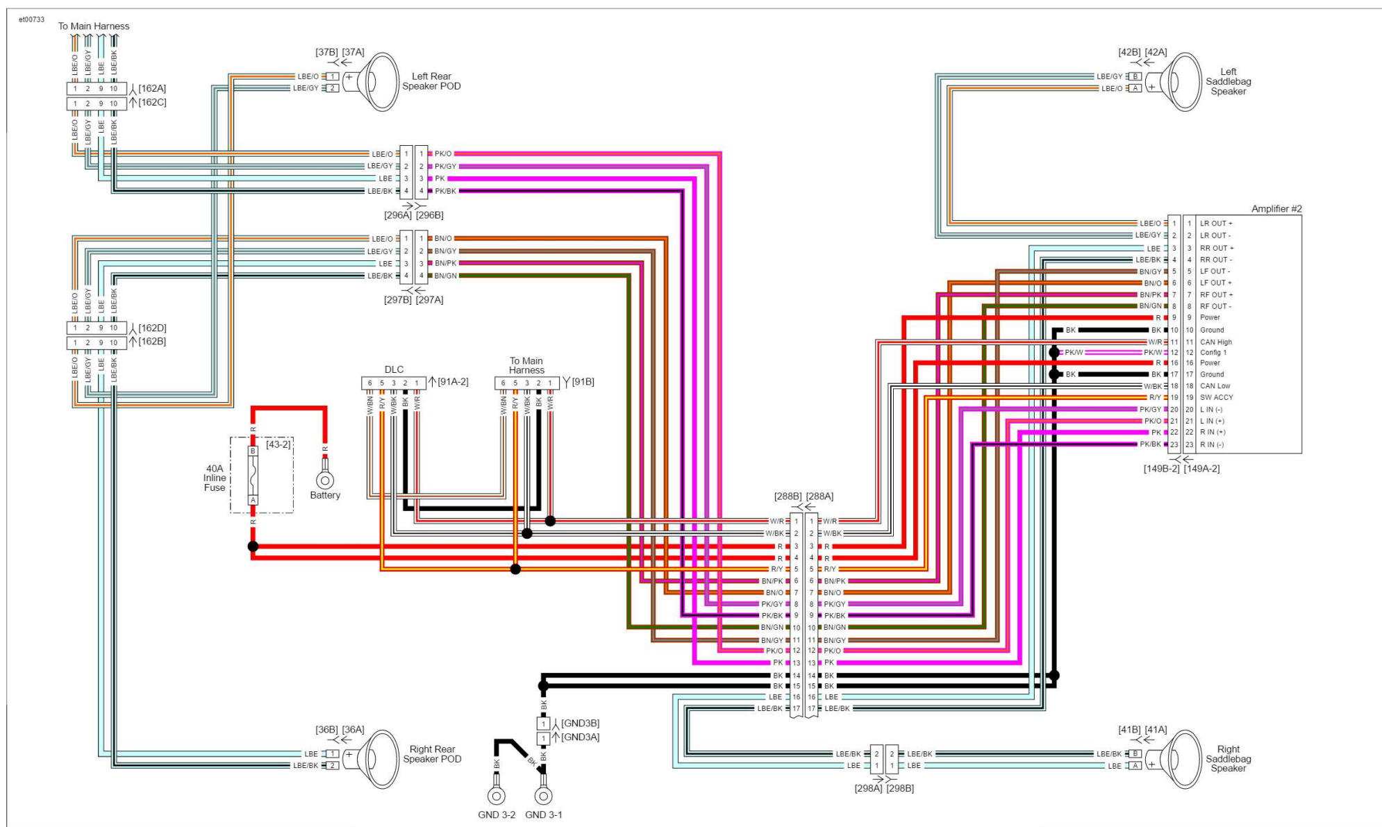
P&amp;A Radio with 2 Amps (2 of 2): 2016 Touring
