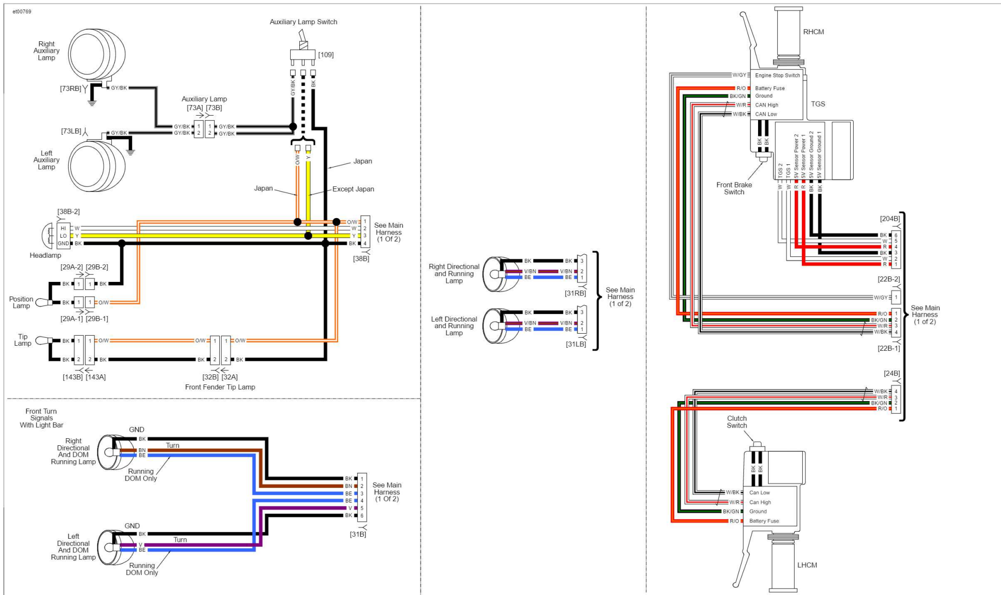
Front Lighting and Hand Controls: 2016 Softail
