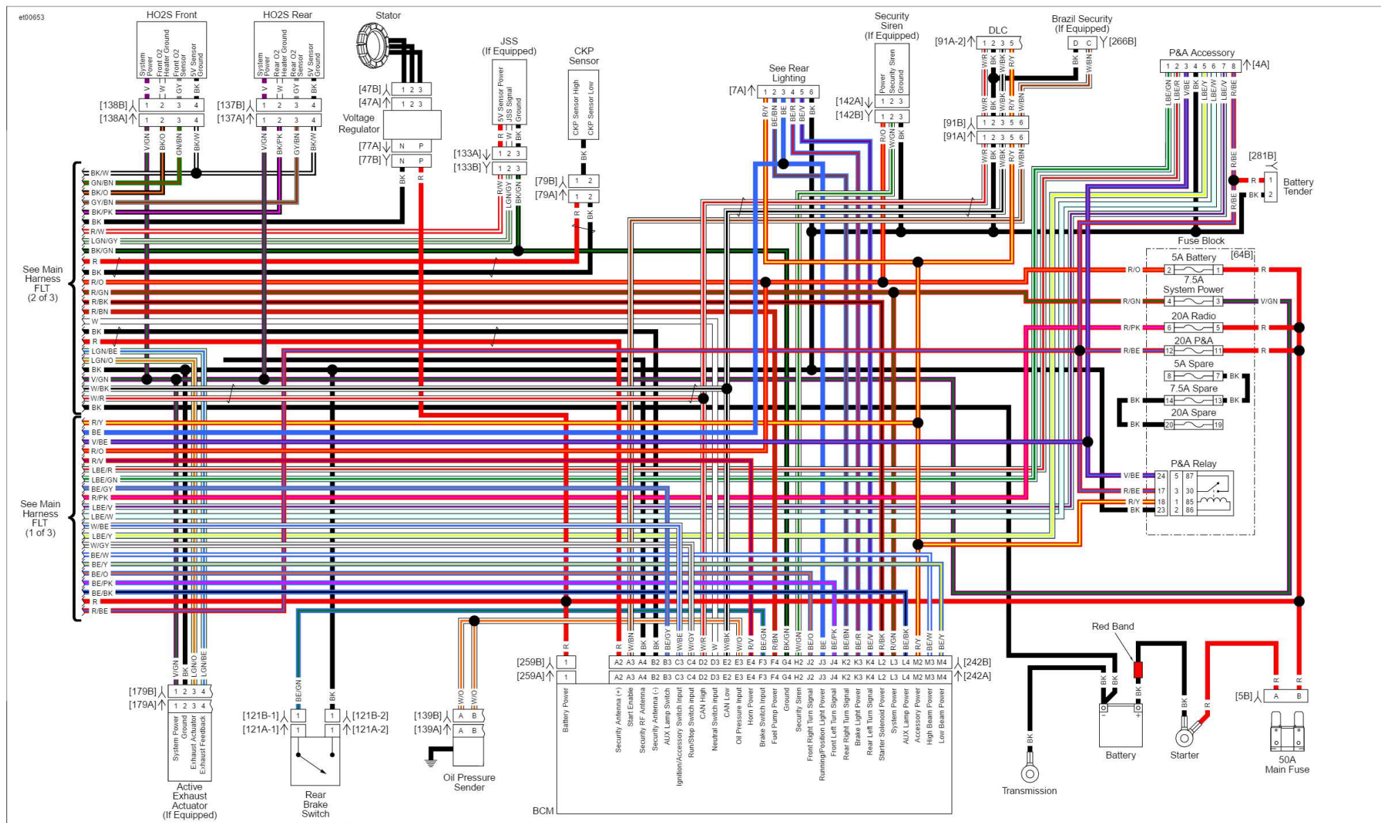
Main Harness FLT (3 of 3): 2016 Touring
