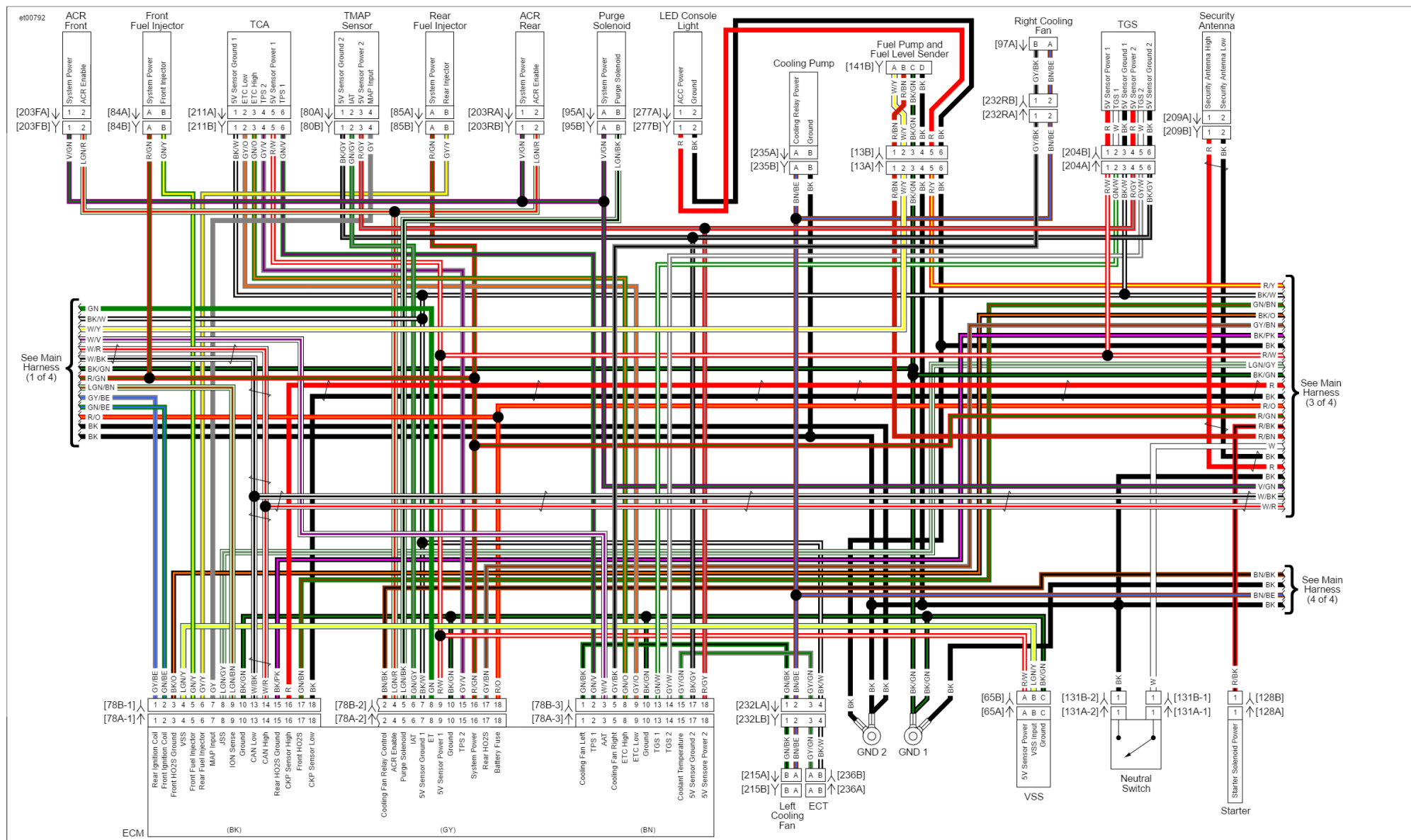
Main Harness (2 of 4): 2016 FLHXSE
