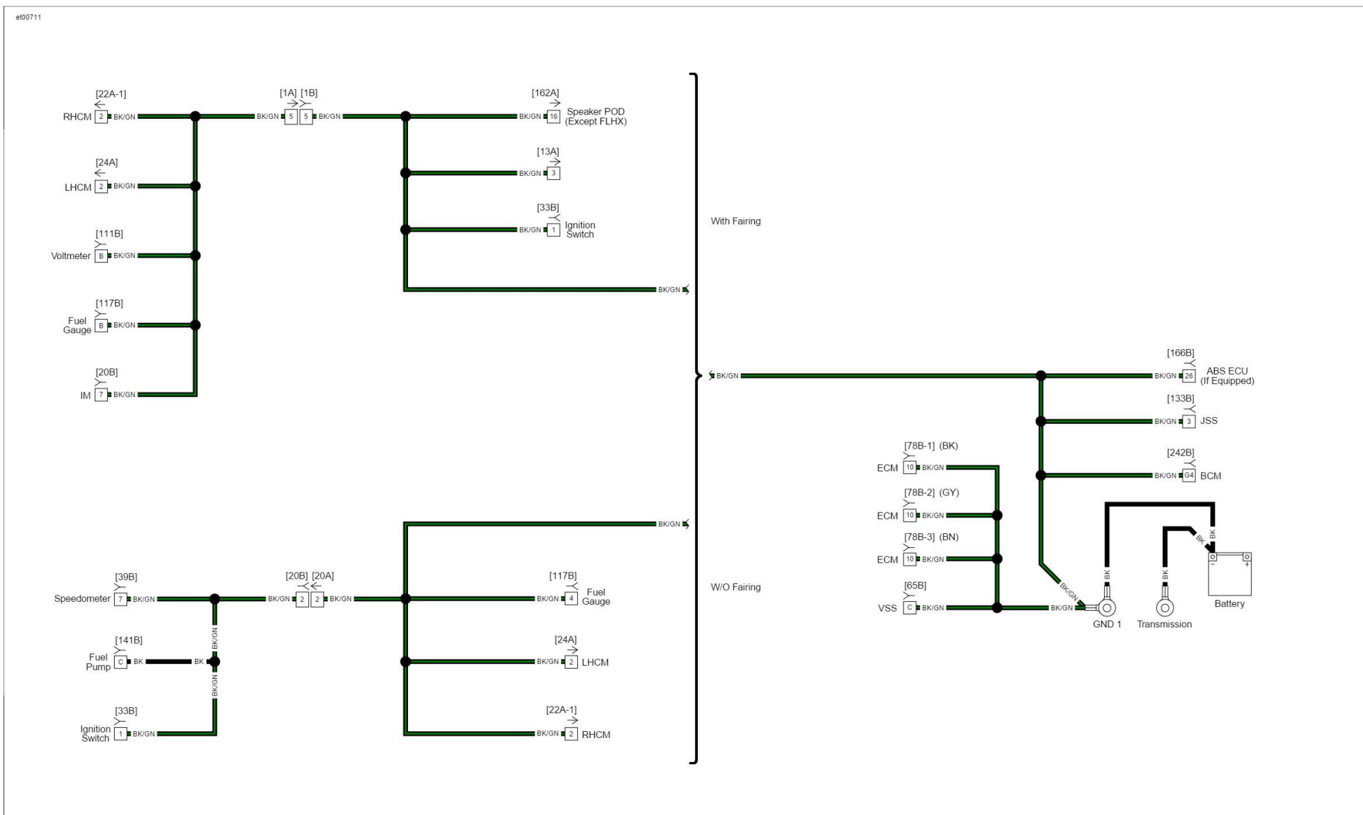
Sensor Grounds FLH: 2016 Touring
