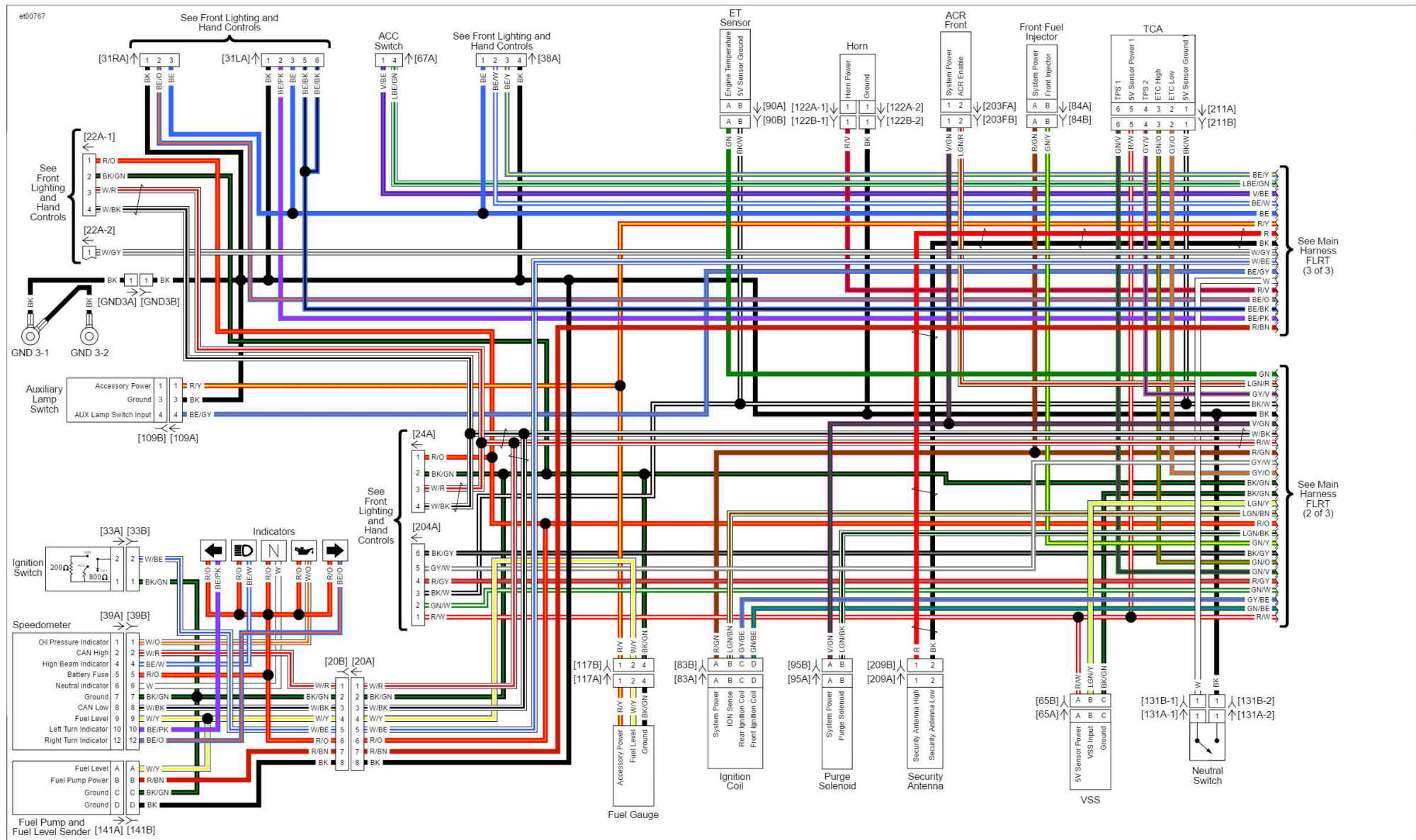
Main Harness FLRT (1 of 3): 2016 Trike Model
