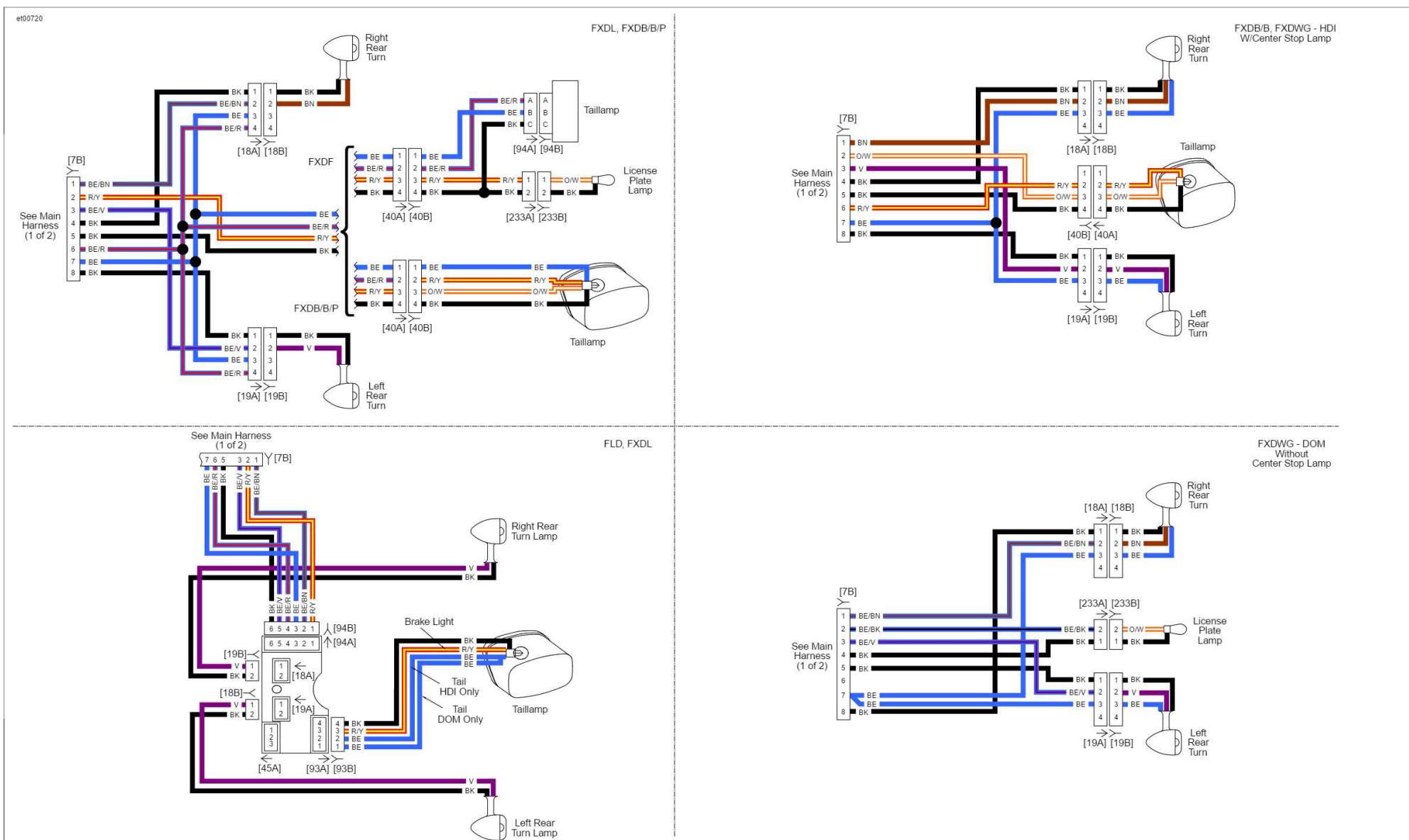
Rear Lighting: 2016 Dyna
