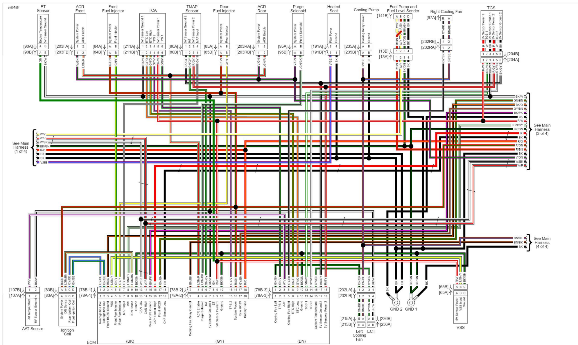
Main Harness (2 of 4): 2016 FLTRUSE
