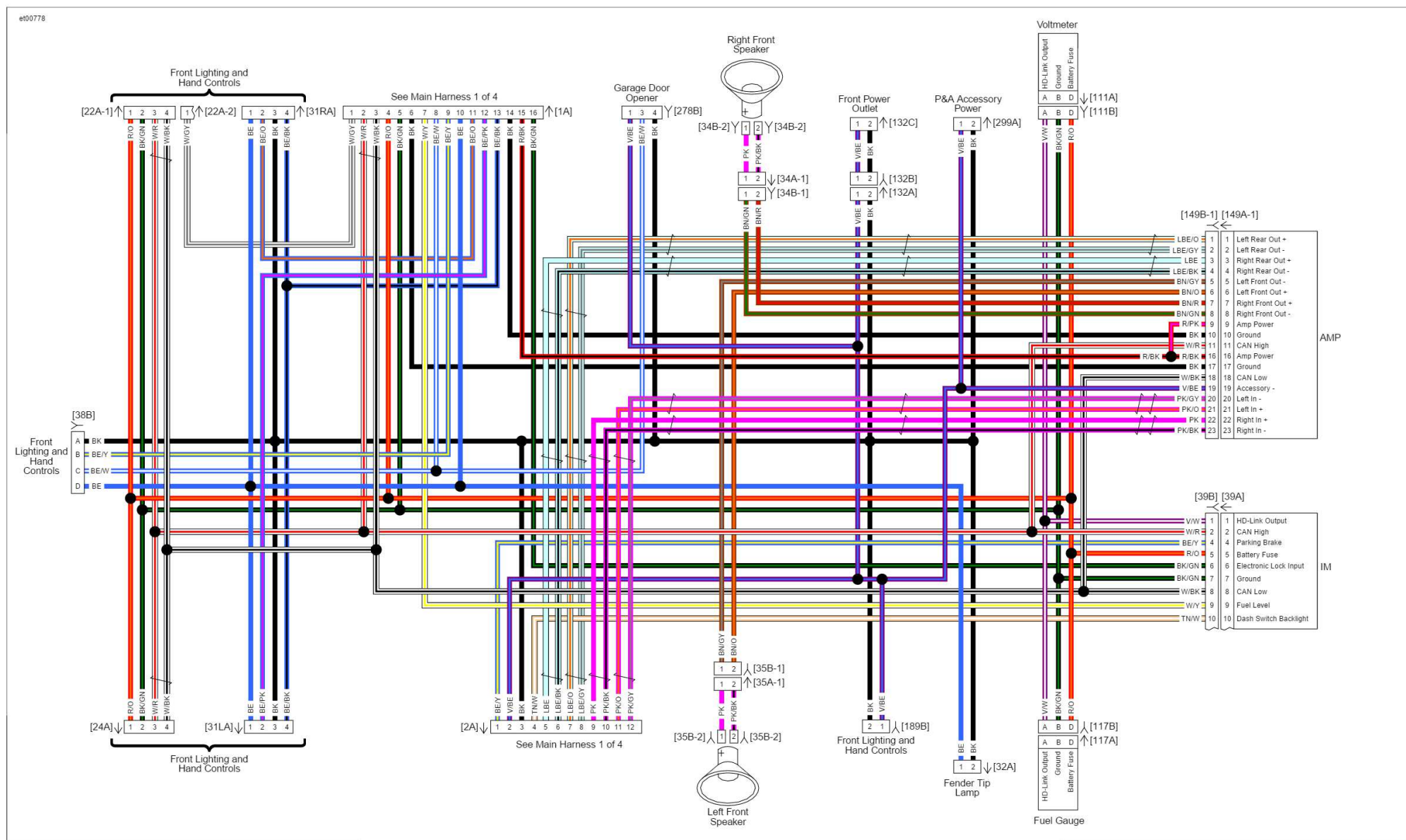
Fairing Harness: 2016 FLHTKSE
