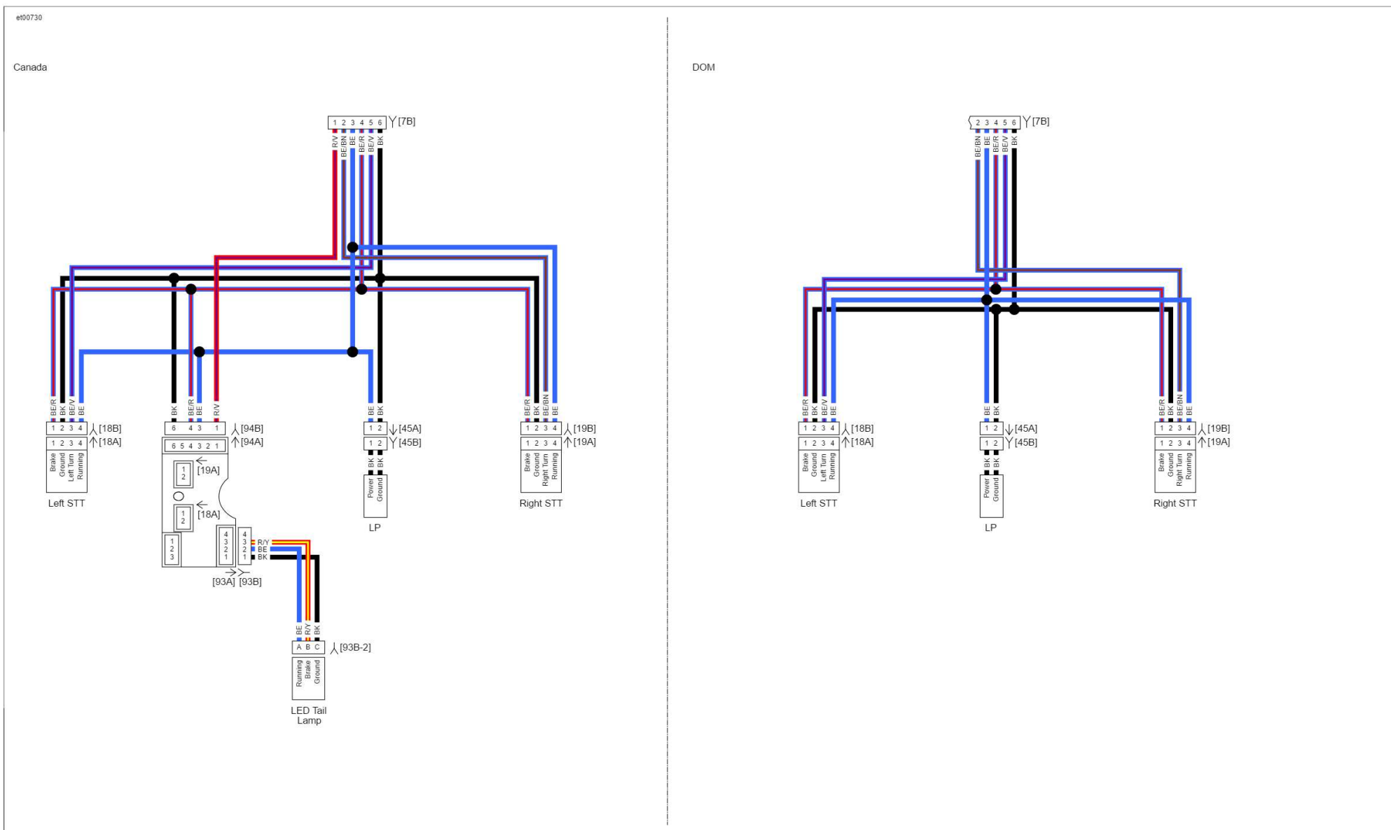
Rear Lighting: 2016 FLHXSE
