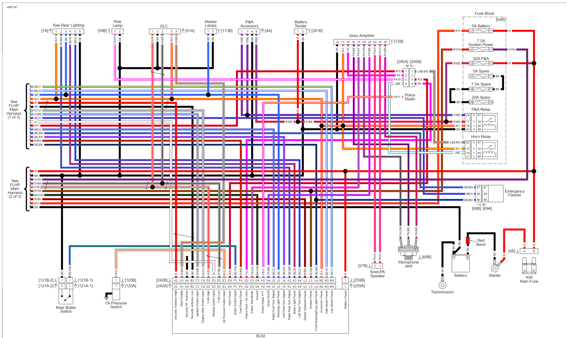
Main Harness (3 of 3): 2016 FLHP
