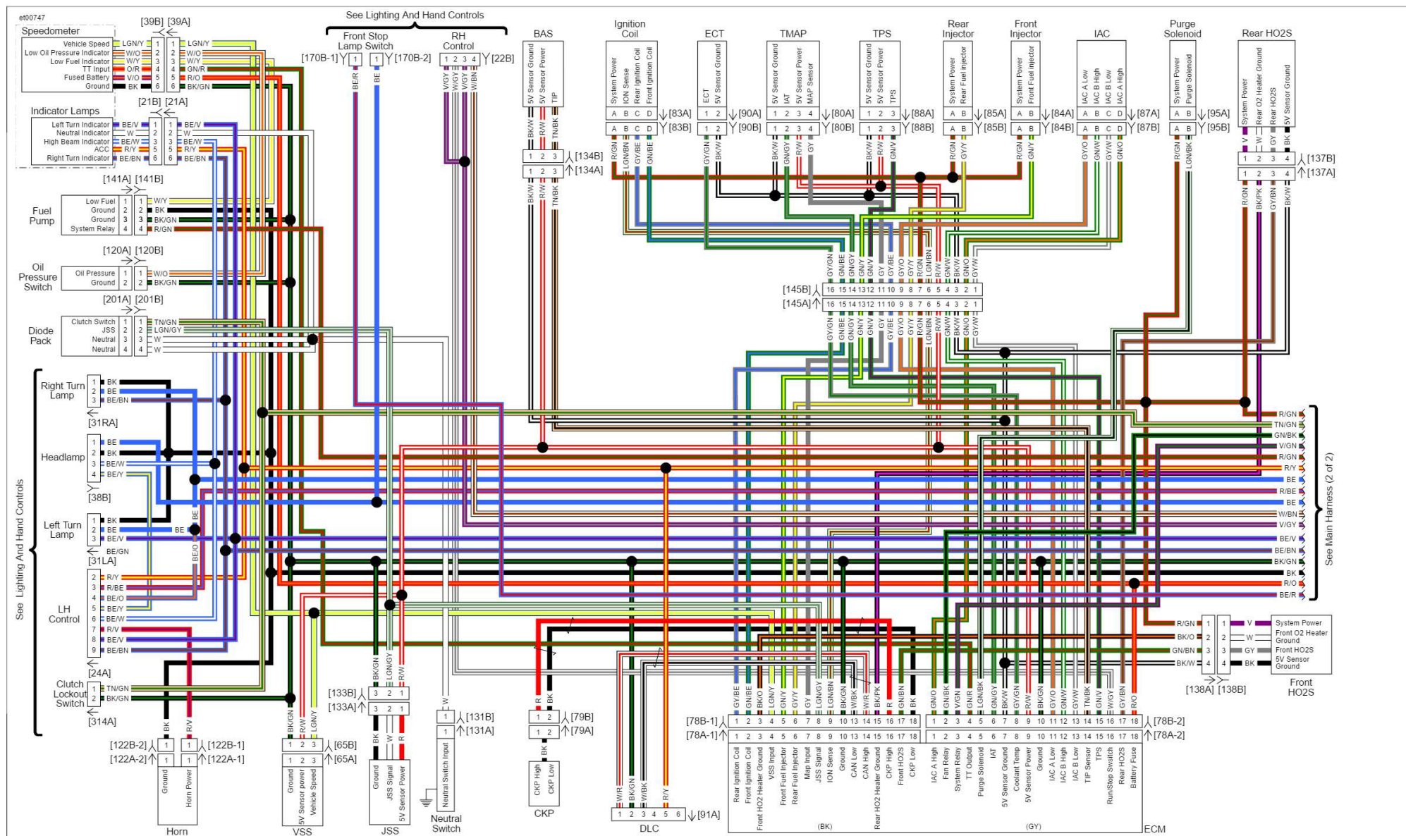
Main Harness (1 of 2): 2016 Street
