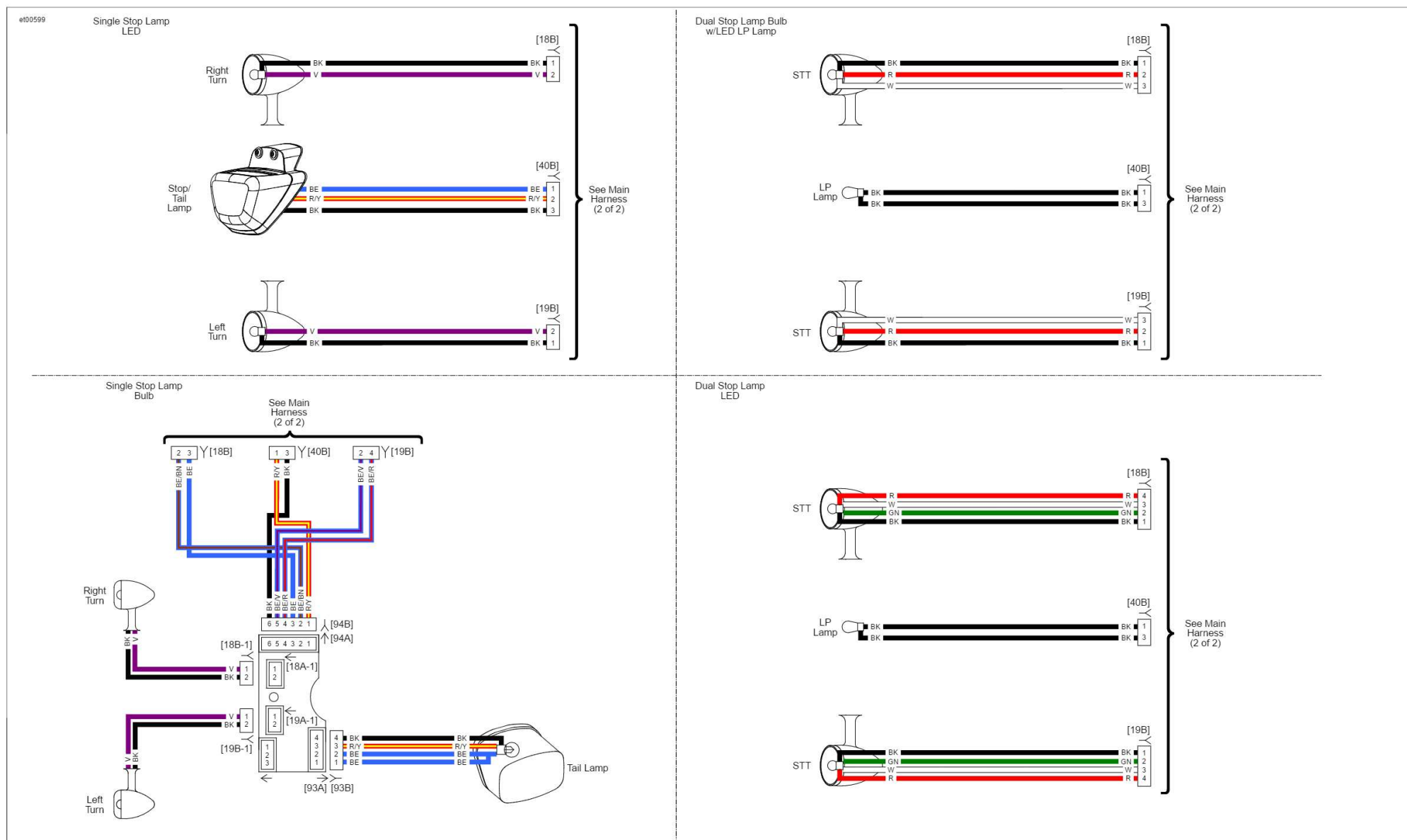
Rear Lighting: 2016 Sportster
