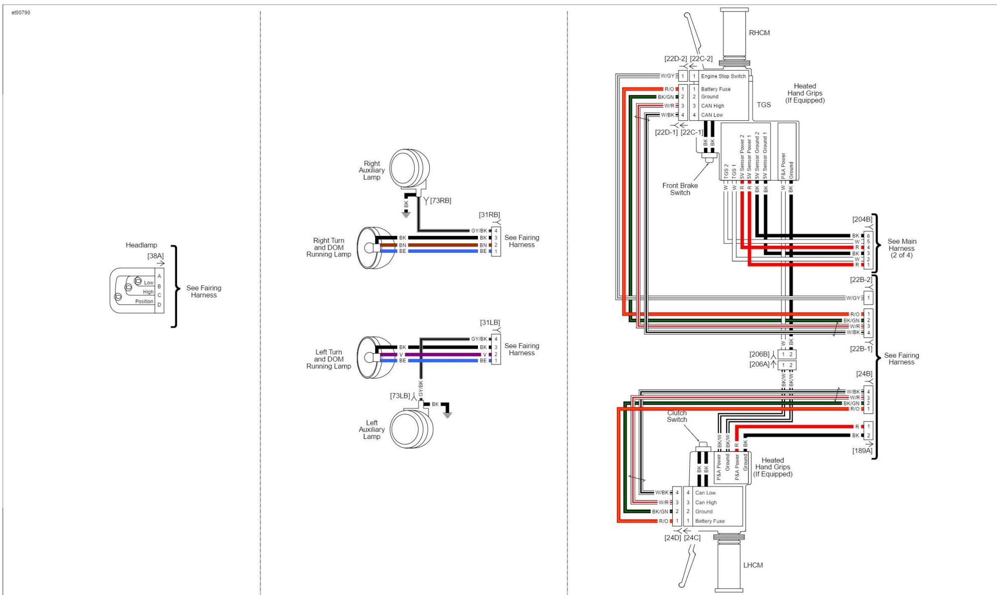
Front Lighting and Hand Controls: 2016 FLHXSE
