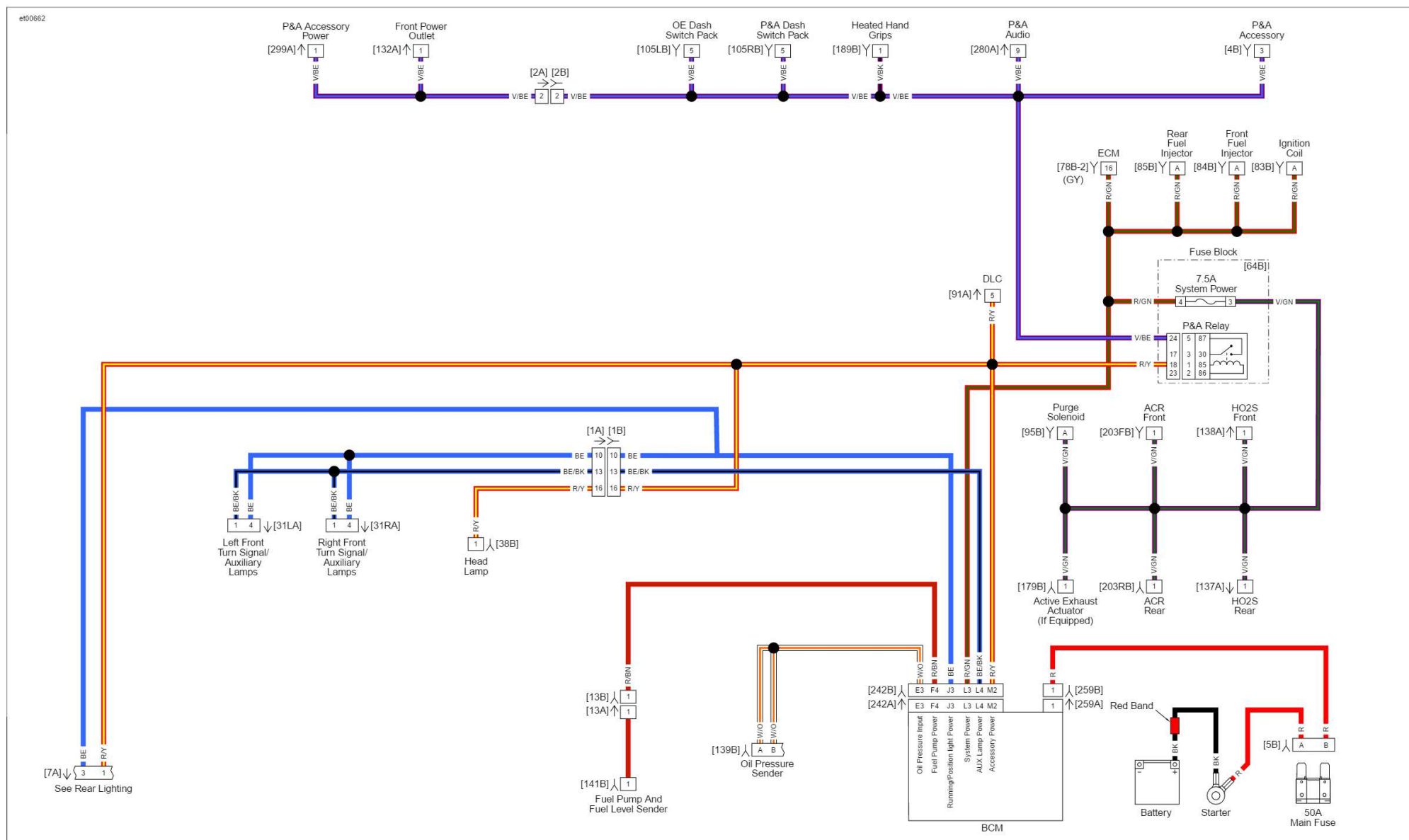
Ignition and ACC FLT: 2016 Touring
