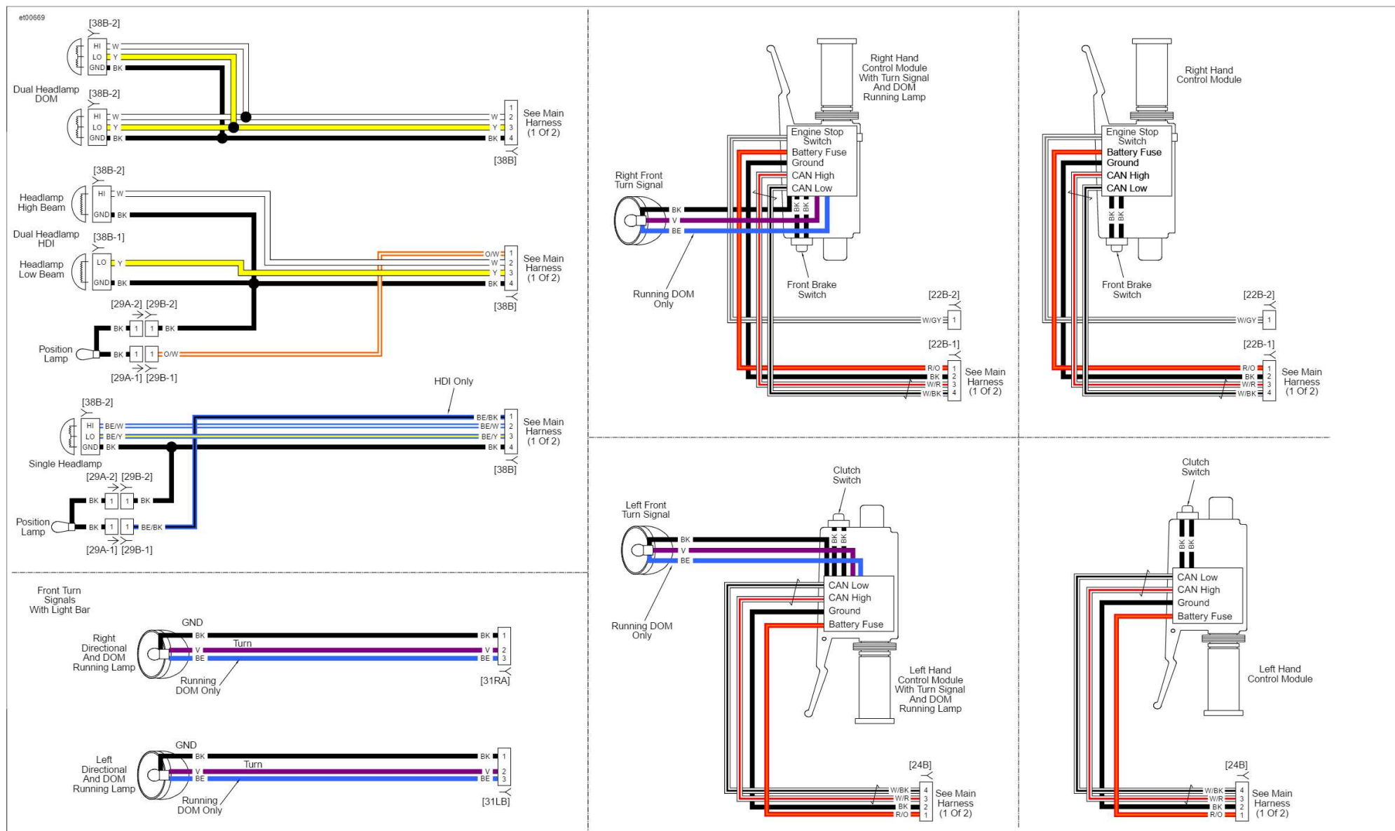
Front Lighting and Hand Controls: 2016 Dyna
