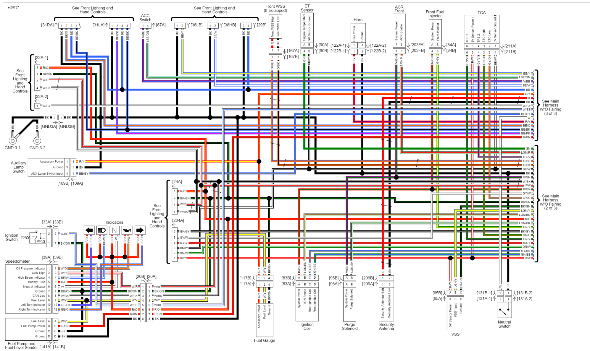
Main Harness (1 of 3): 2016 Touring (without Fairing)
