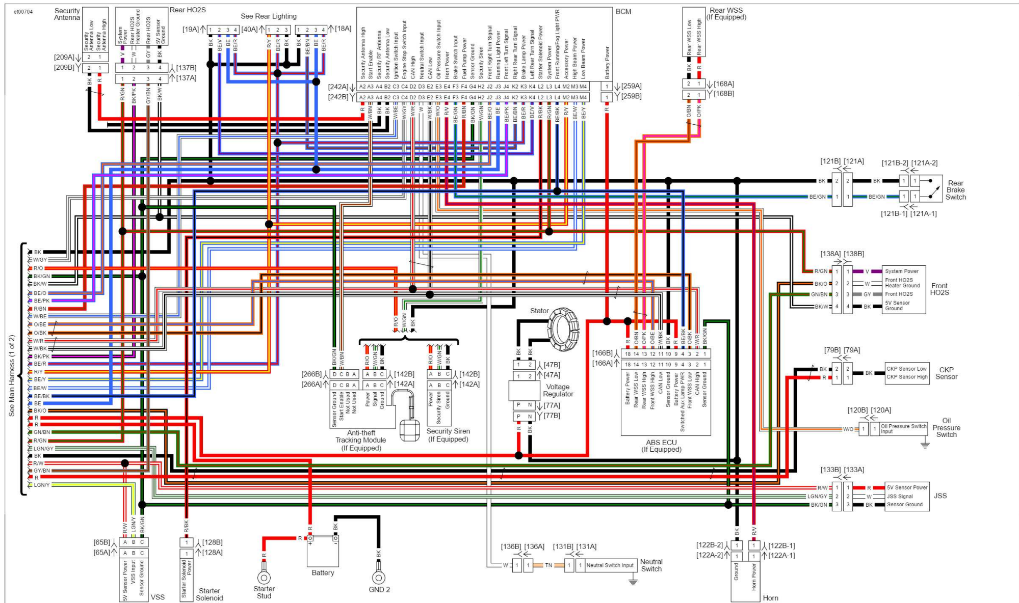
Main Harness 2 of 2: 2016 Sportster
