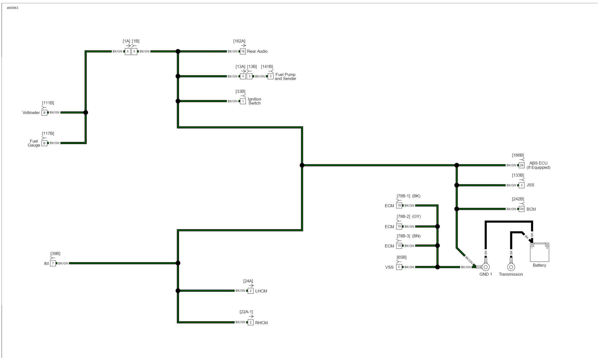
Sensor Grounds FLT: 2016 Touring
