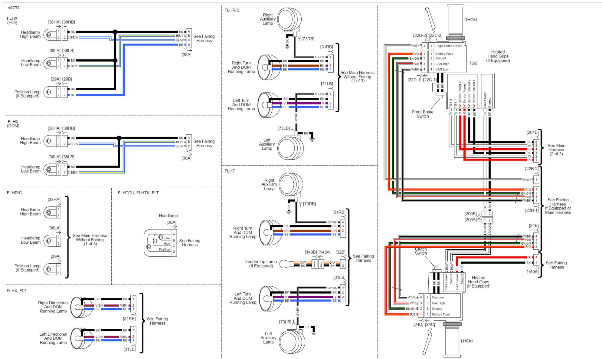
Front Lighting and Hand Controls: 2016 Touring
