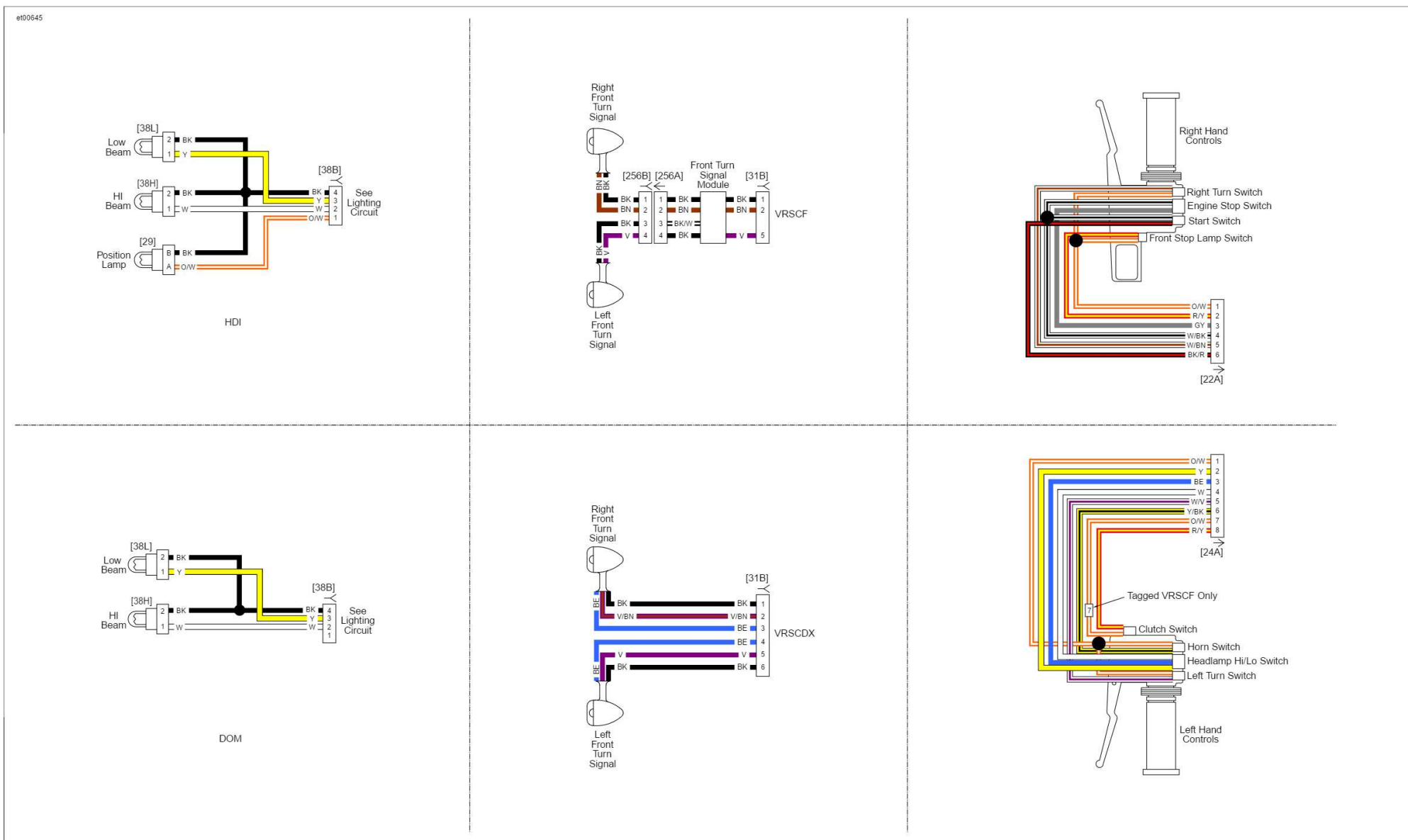
Front Lighting and Hand Controls: 2016 V-Rod
