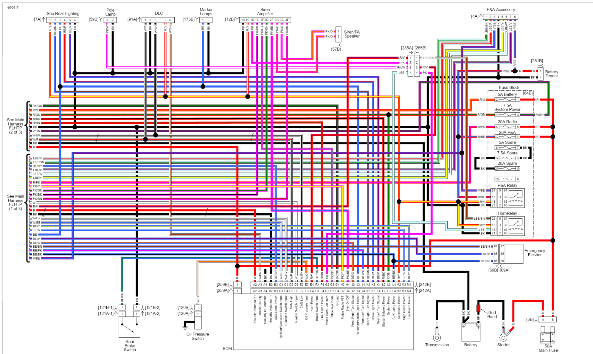
Main Harness (3 of 3): 2016 FLHTP
