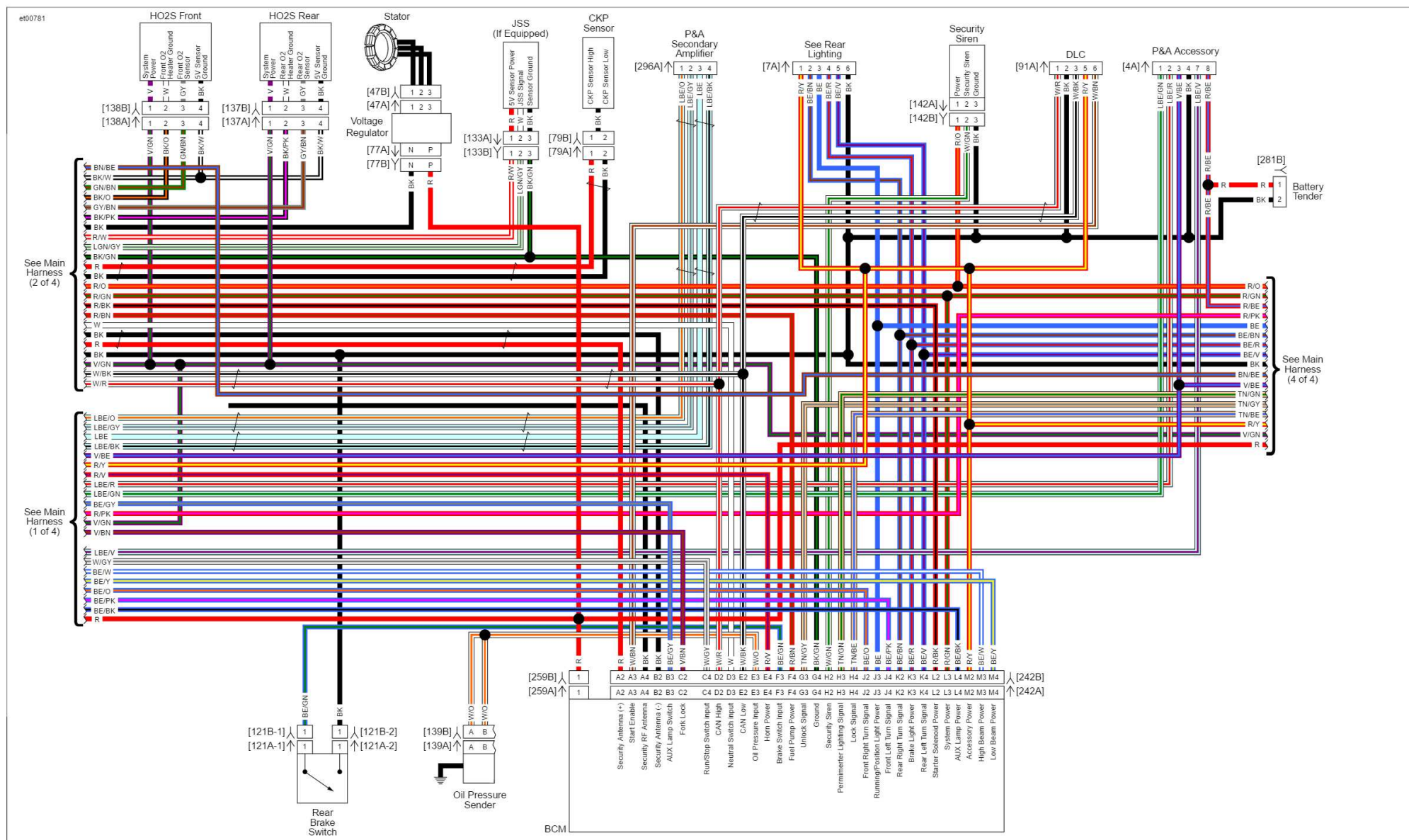
Main Harness (3 of 4): 2016 FLHTKSE
