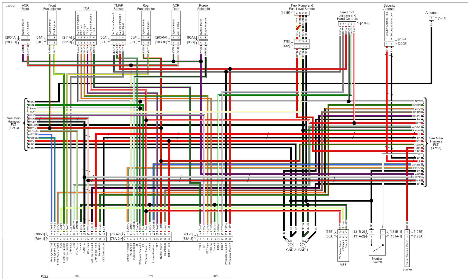
Main Harness FLT (2 of 3): 2016 Touring
