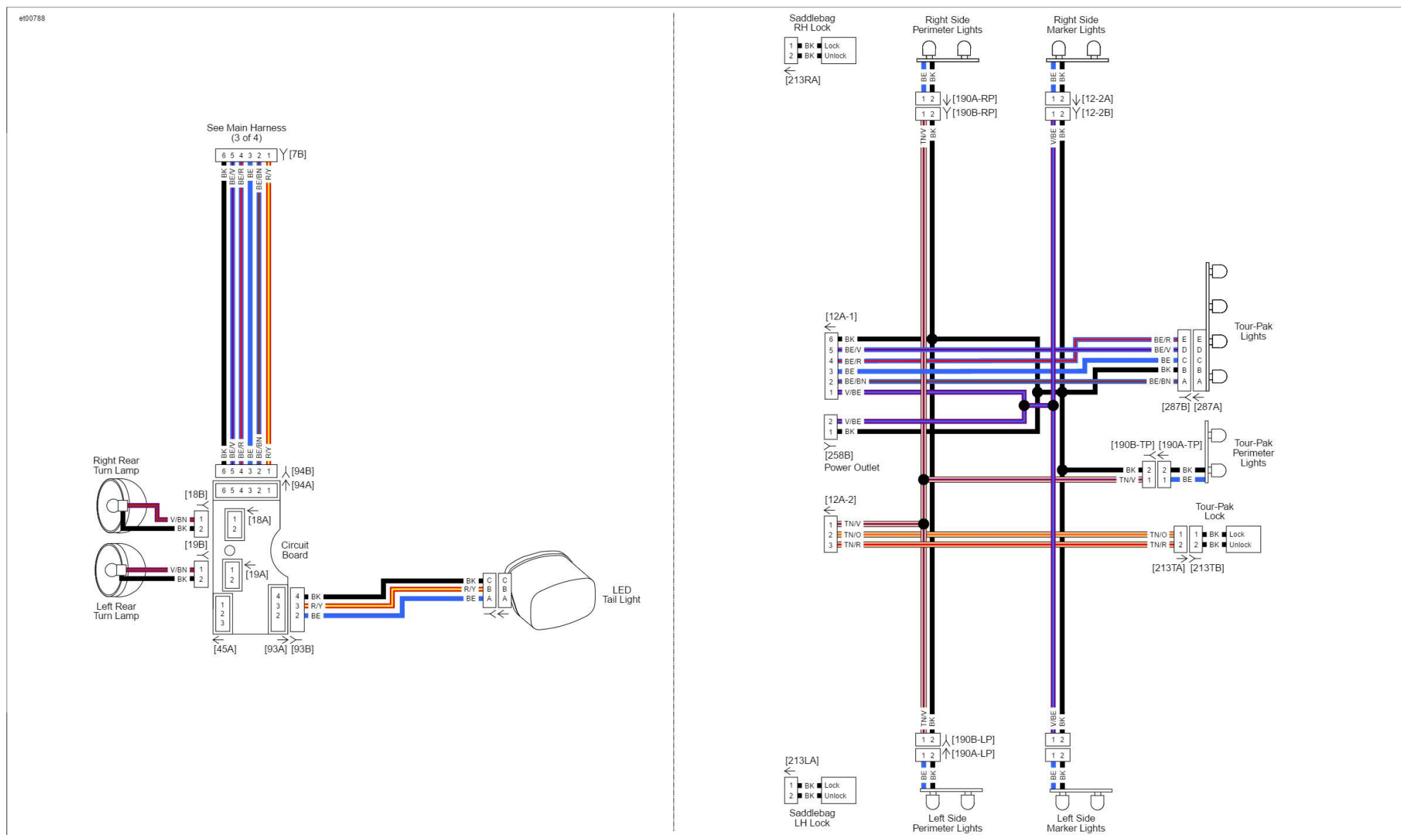
Rear Lighting: 2016 FLTRUSE
