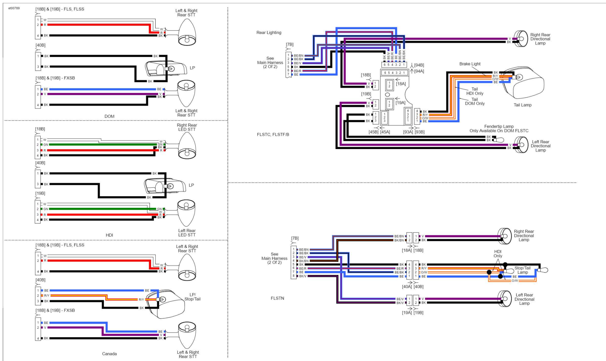
Rear Lighting: 2016 Softail
