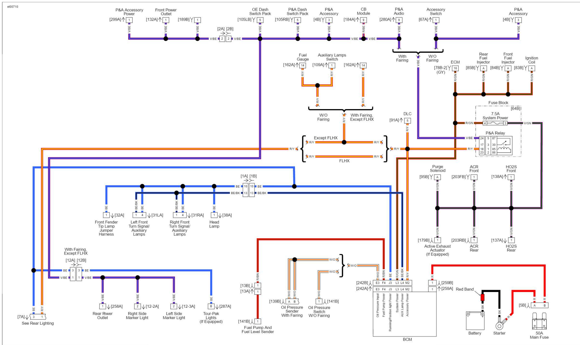
Ignition and ACC FLH: 2016 Touring
