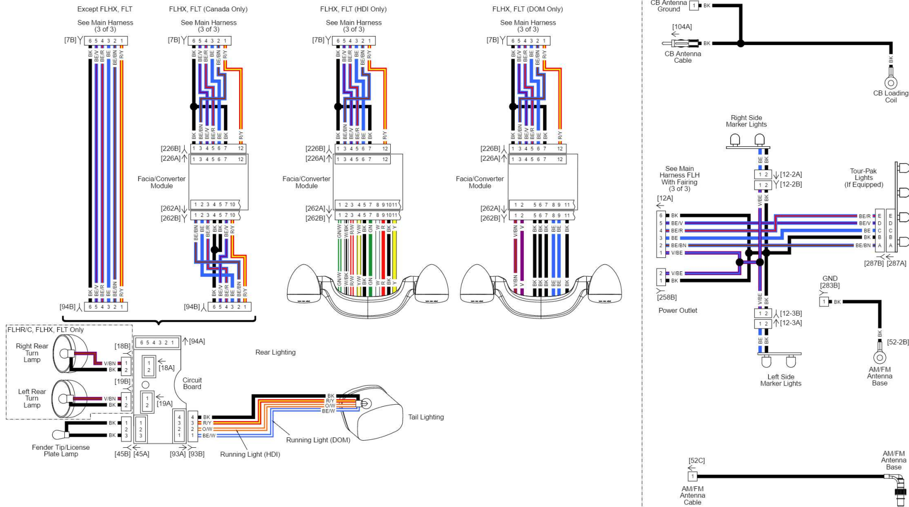
Rear Lighting: 2016 Touring
