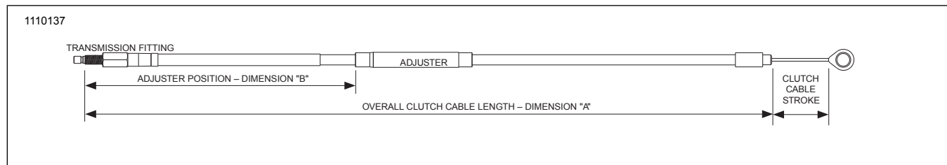
Figure 50. Clutch Cables
