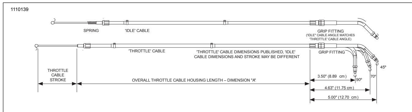
Figure 52. Throttle/Idle Cables
