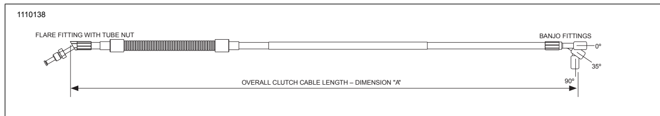
Figure 51. Hydraulic Clutch Lines
