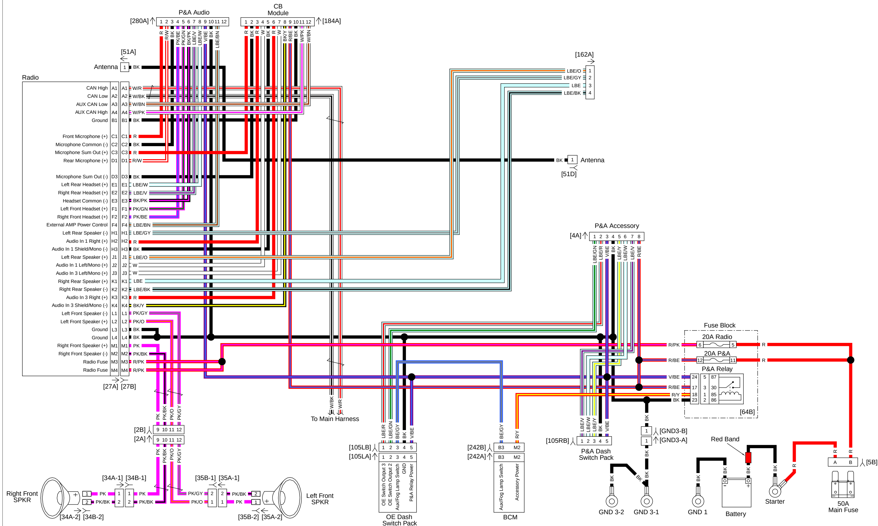
OE Radio: 2015 Touring (FLT)
