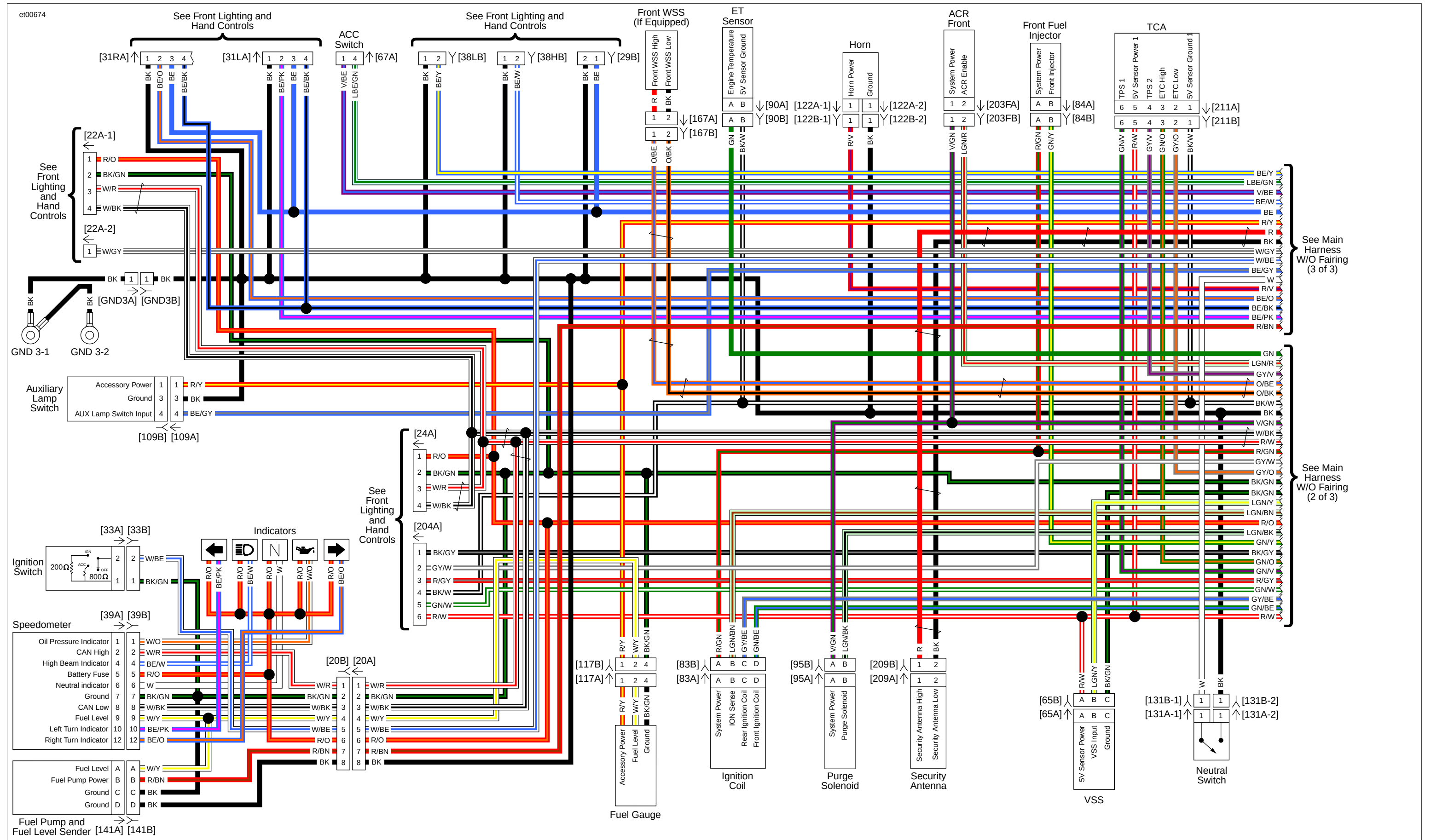
Main Harness (1 of 3): 2015 Touring (Without Fairing)
