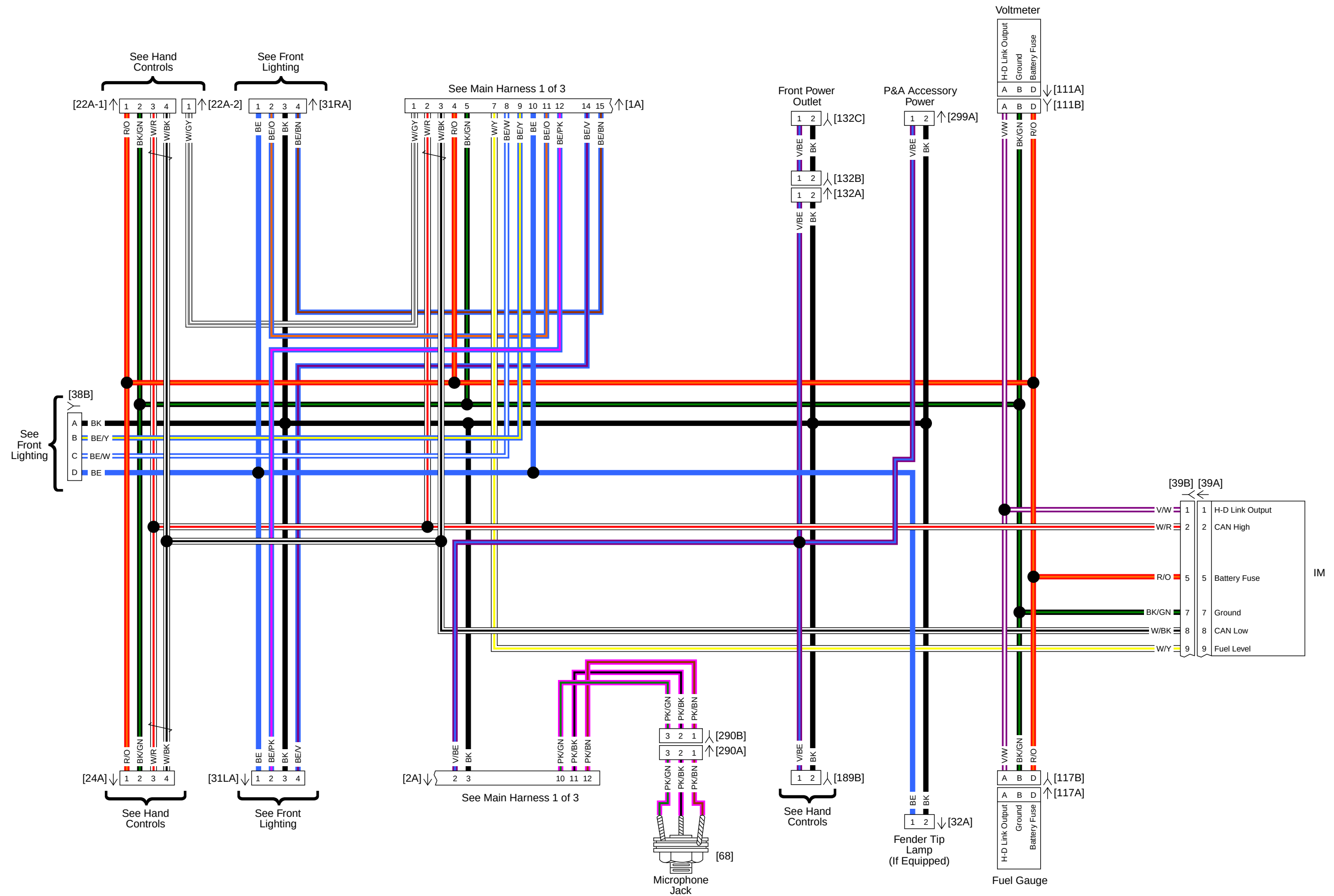
Fairing Harness: 2015 FLHTP
