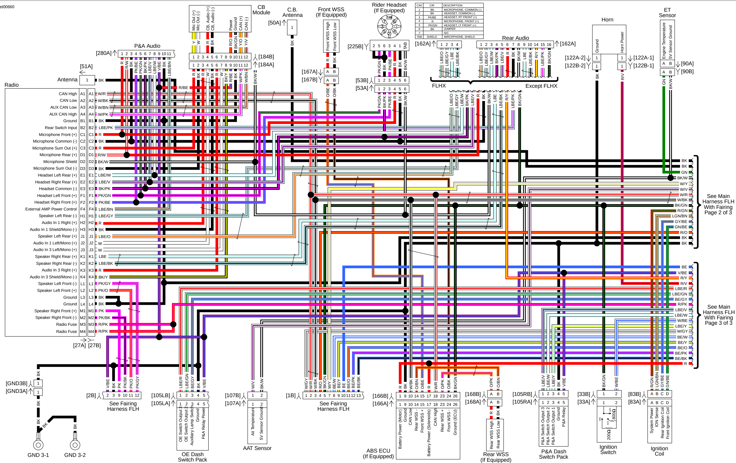
Main Harness FLH (1 of 3): 2015 Touring (With Fairing)
