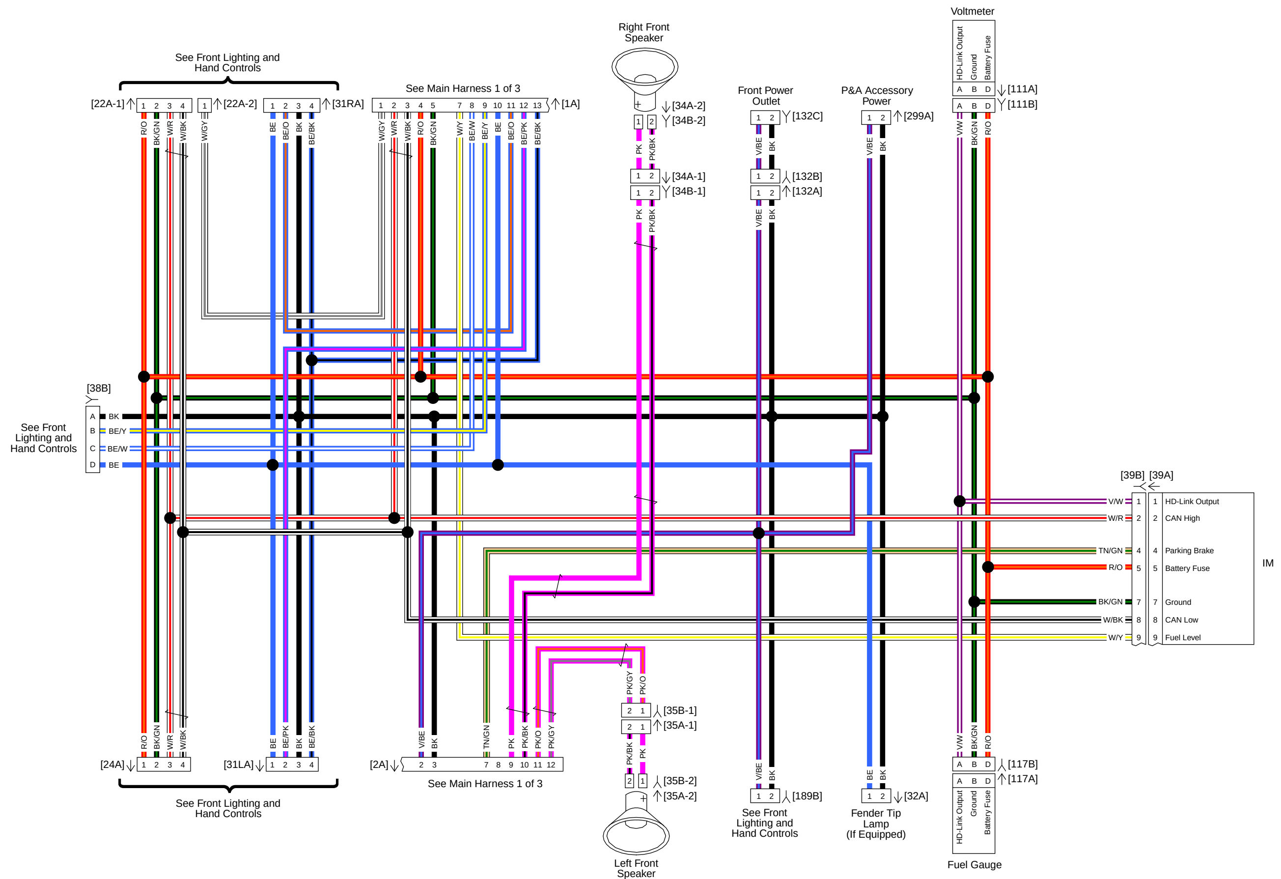
Fairing Harness FLH: 2015 Touring
