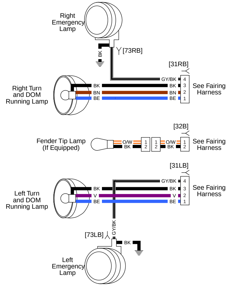
Front Lighting and Hand Controls: 2015 Police
