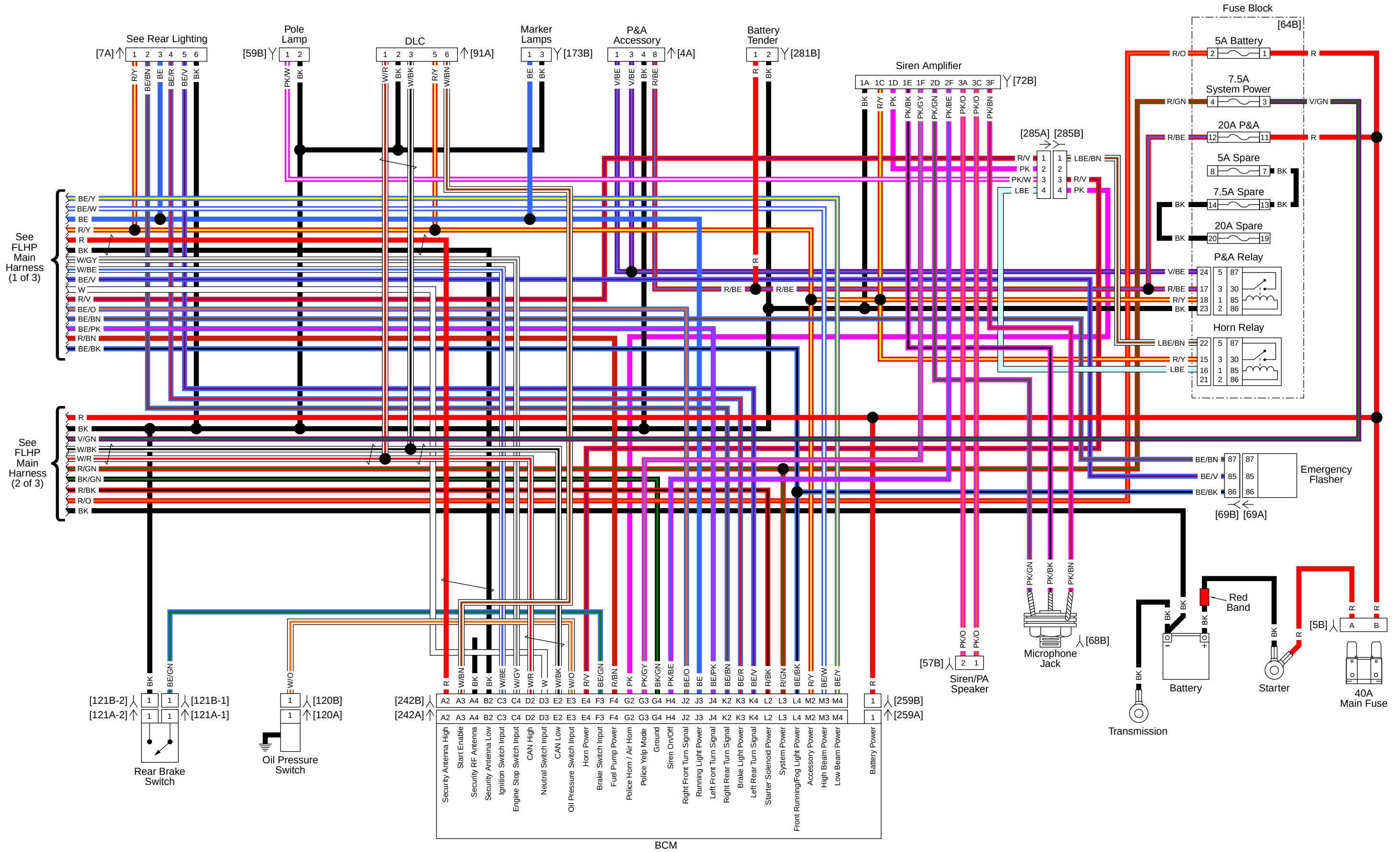
Main Harness (3 of 3): 2015 FLHP
