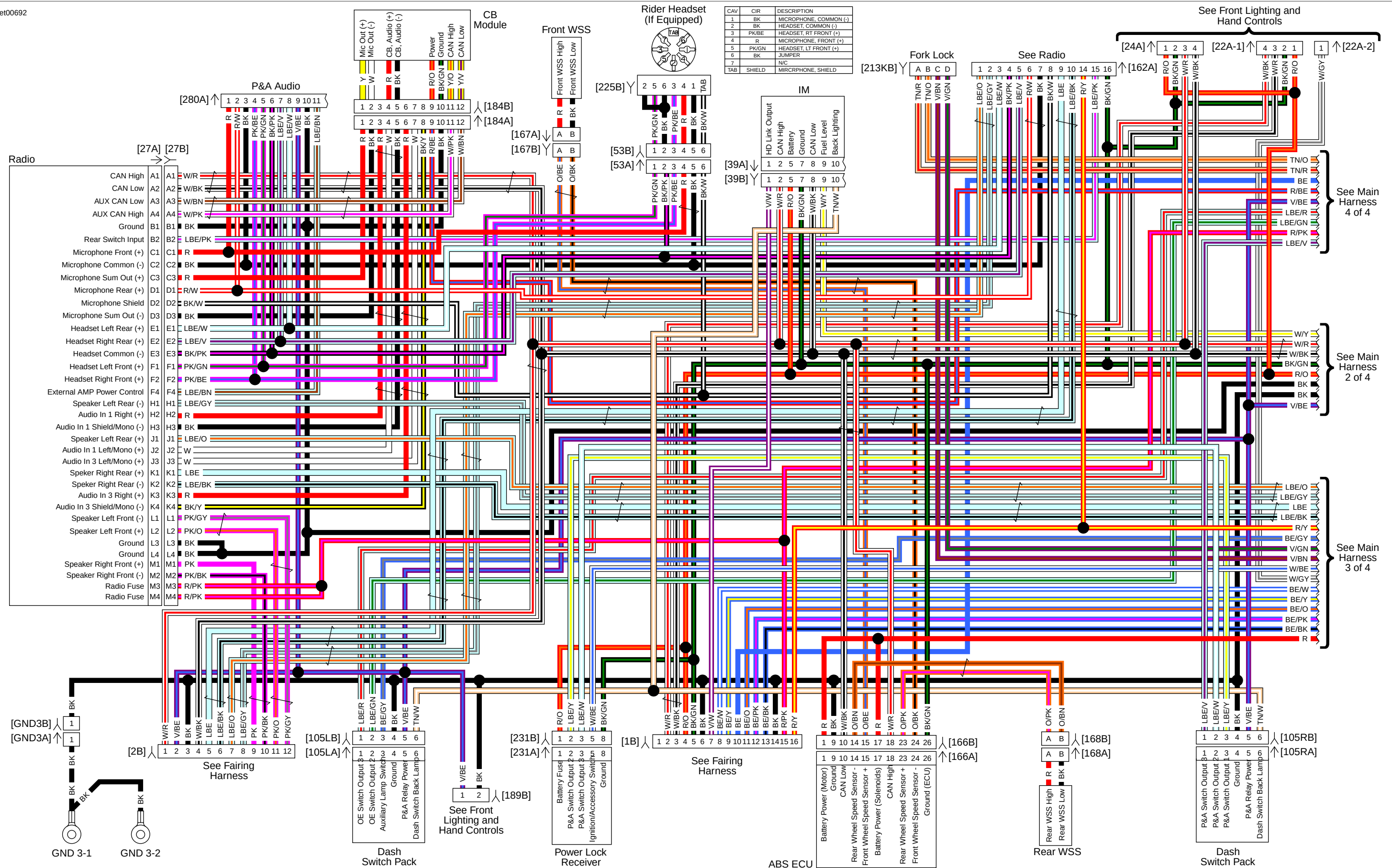
Main Harness (1 of 4): 2015 FLTRUSE
