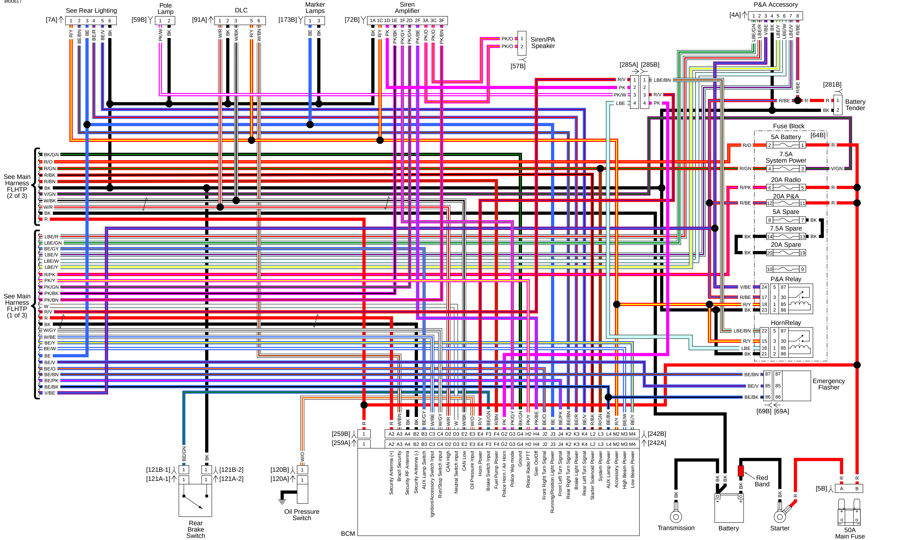
Main Harness (3 of 3): 2015 FLHTP
