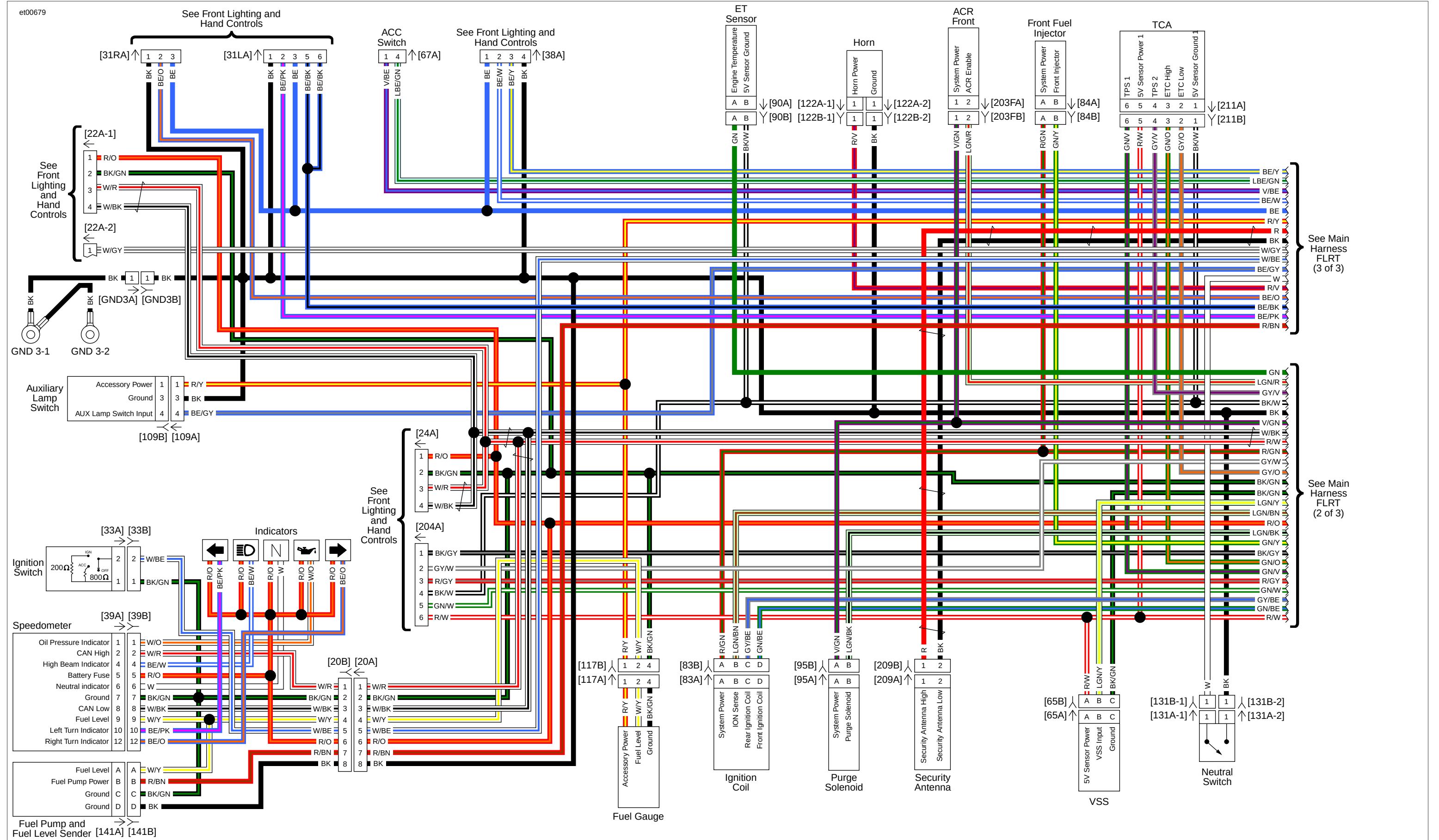
Main Harness FLRT (1 of 3): 2015 Trike Model
