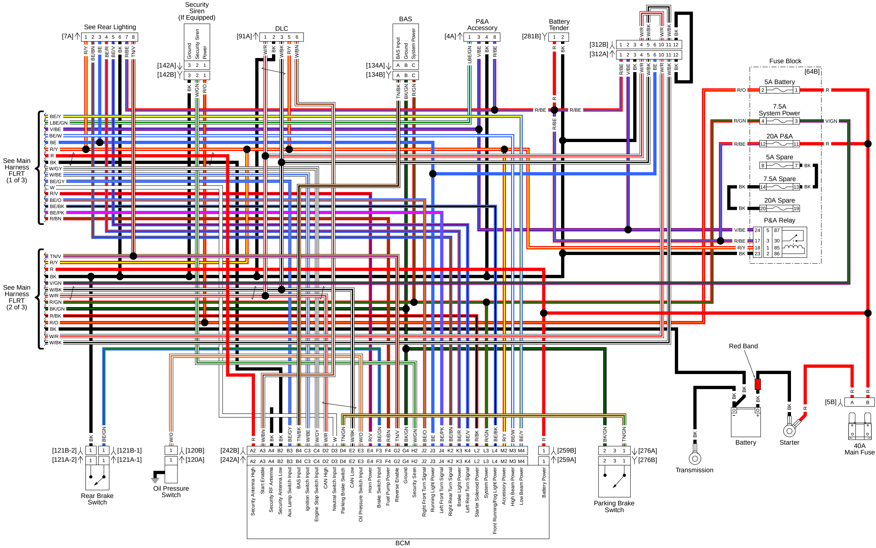
Main Harness FLRT (3 of 3): 2015 Trike Model
