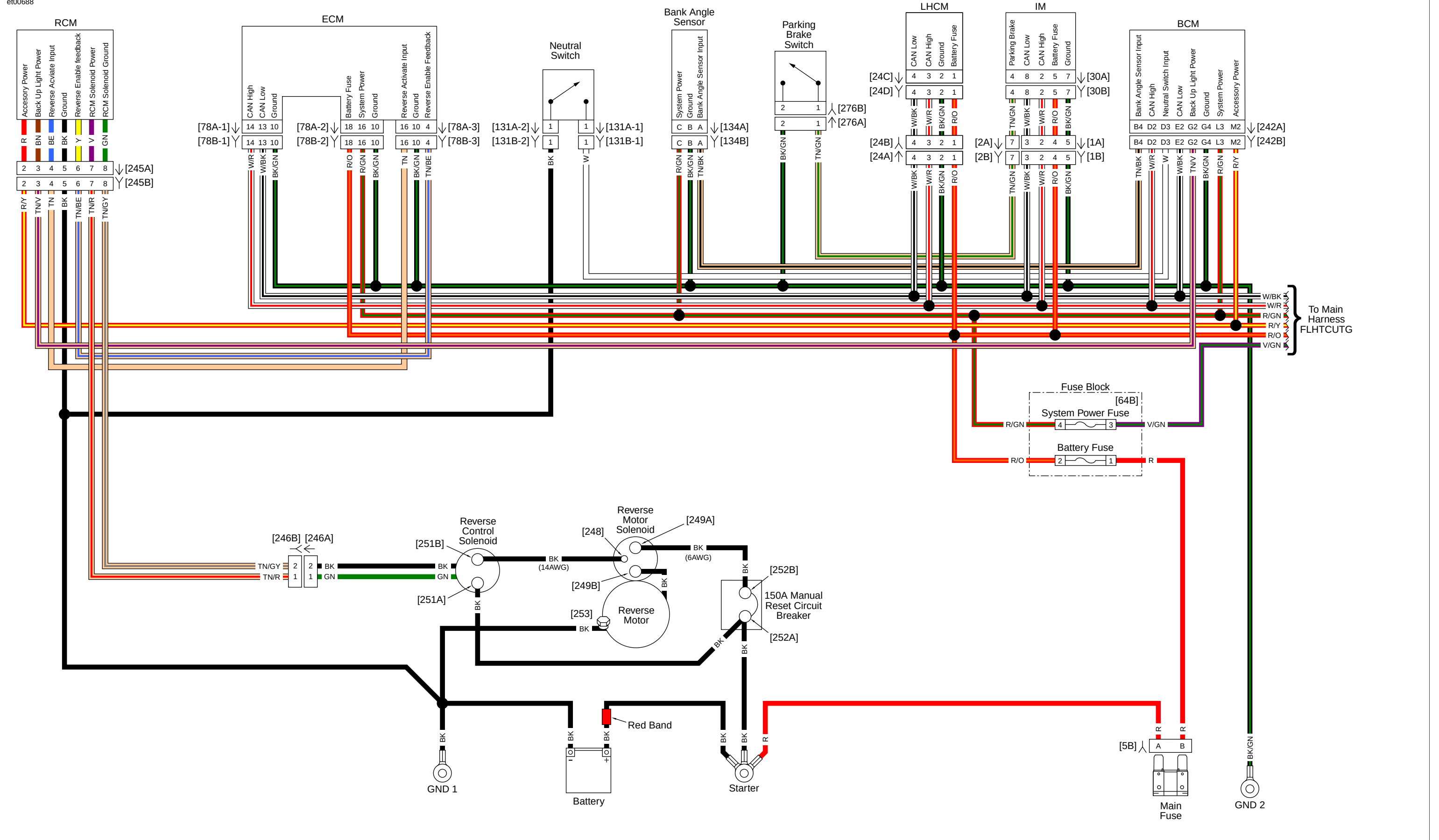
Reverse FLHTCUTG: 2015 Trike Model
