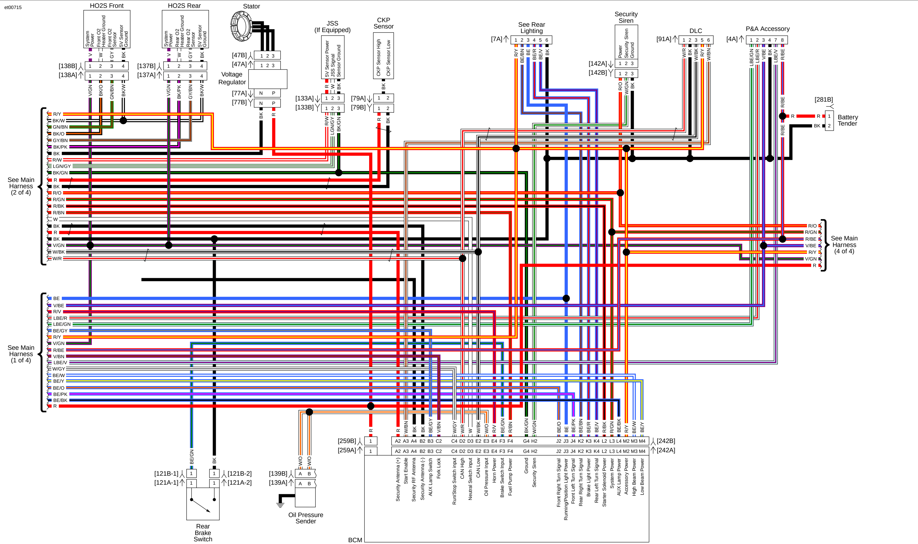
Main Harness (3 of 4): 2015 FLHXSE
