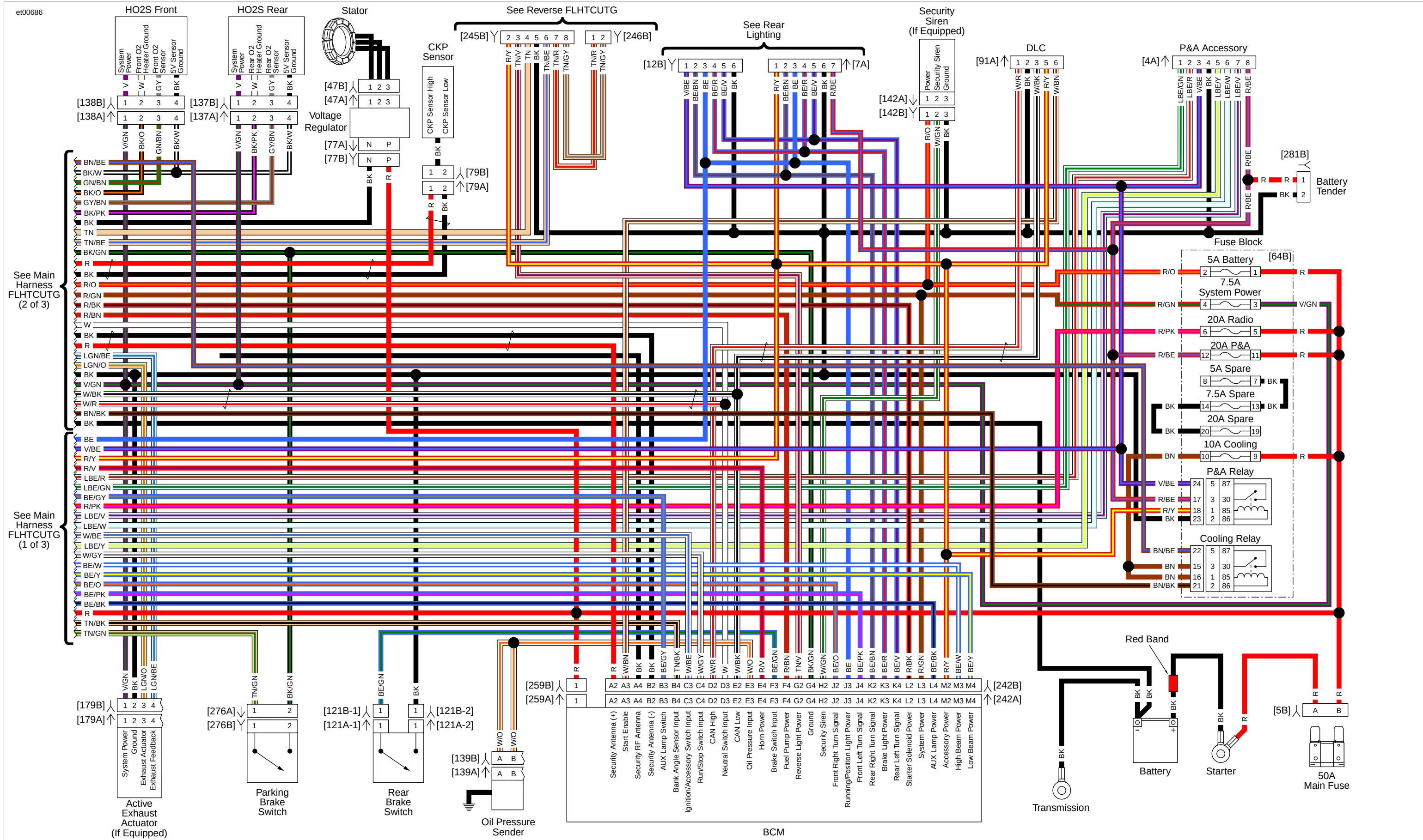
Main Harness FLHTCUTG (3 of 3): 2015 Trike Model
