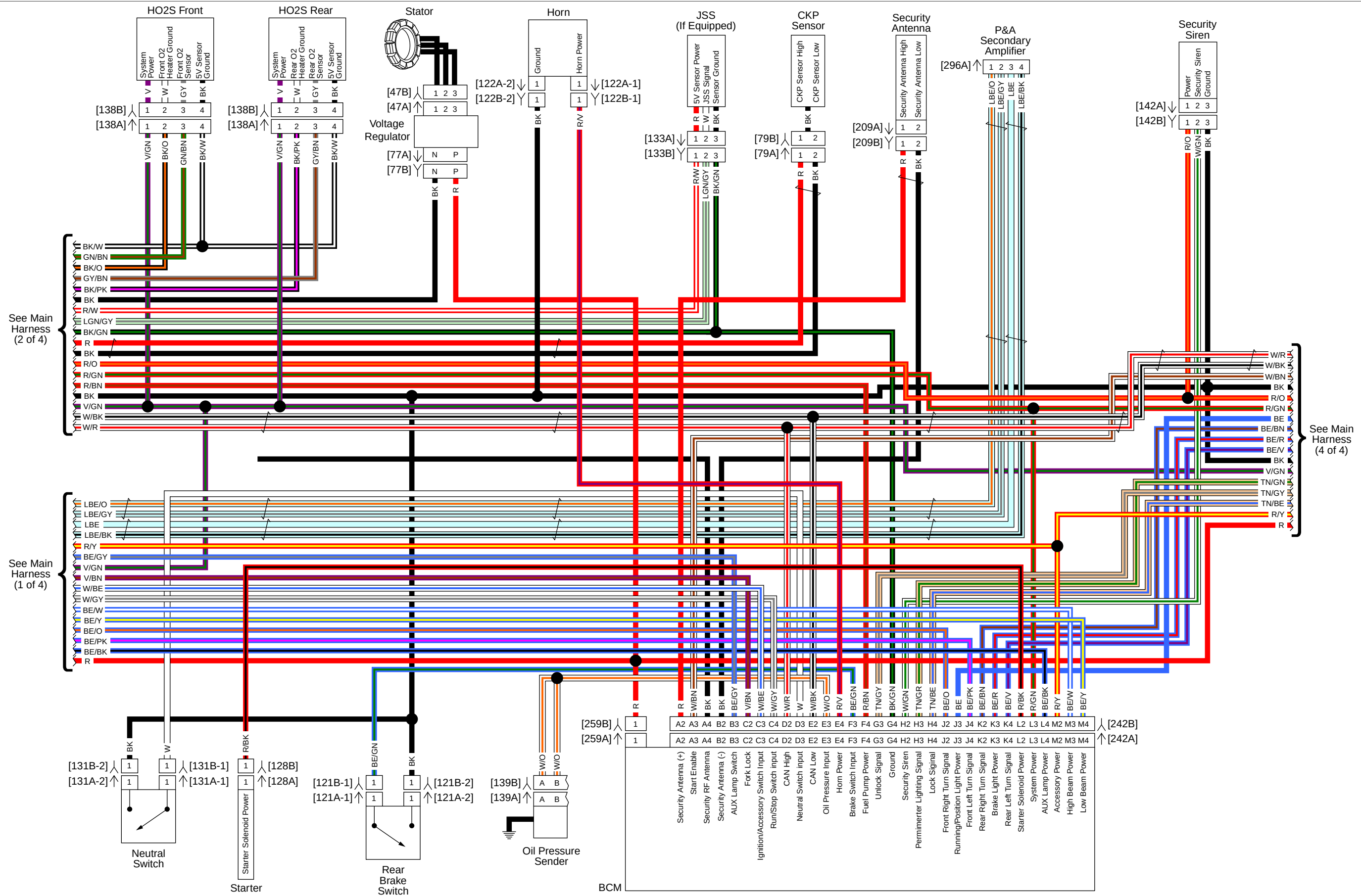
Main Harness (3 of 4): 2015 FLTRUSE
