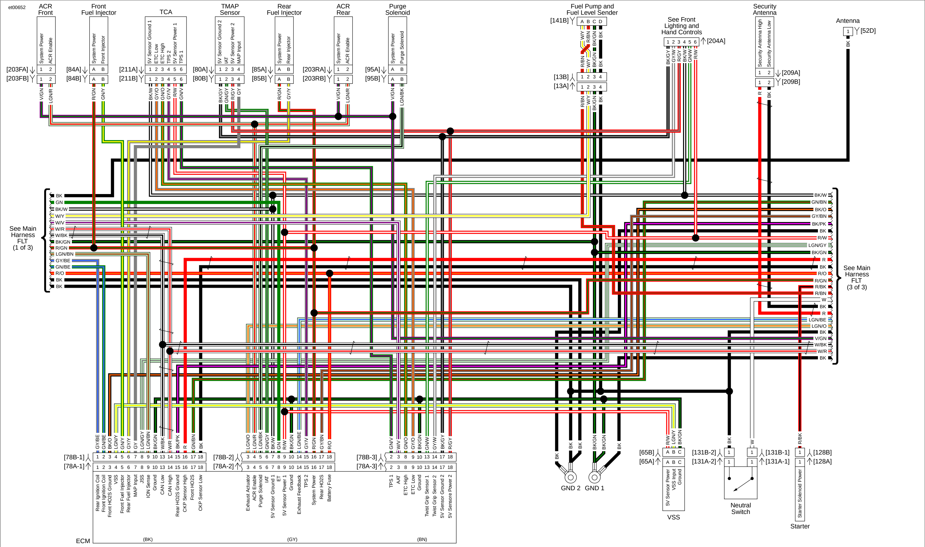
Main Harness FLT (2 of 3): 2015 Touring
