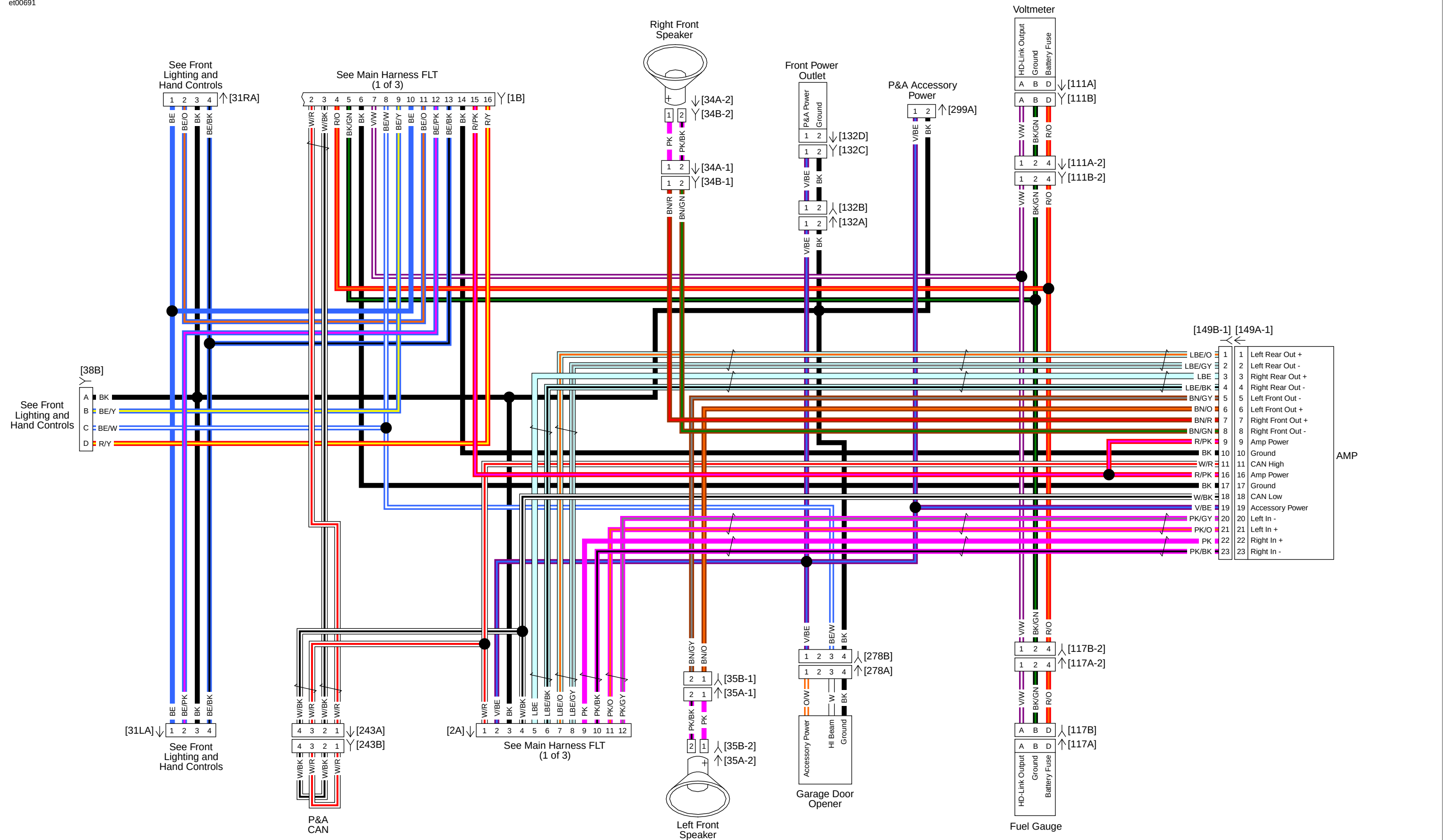
Fairing Harness: 2015 FLTRUSE
