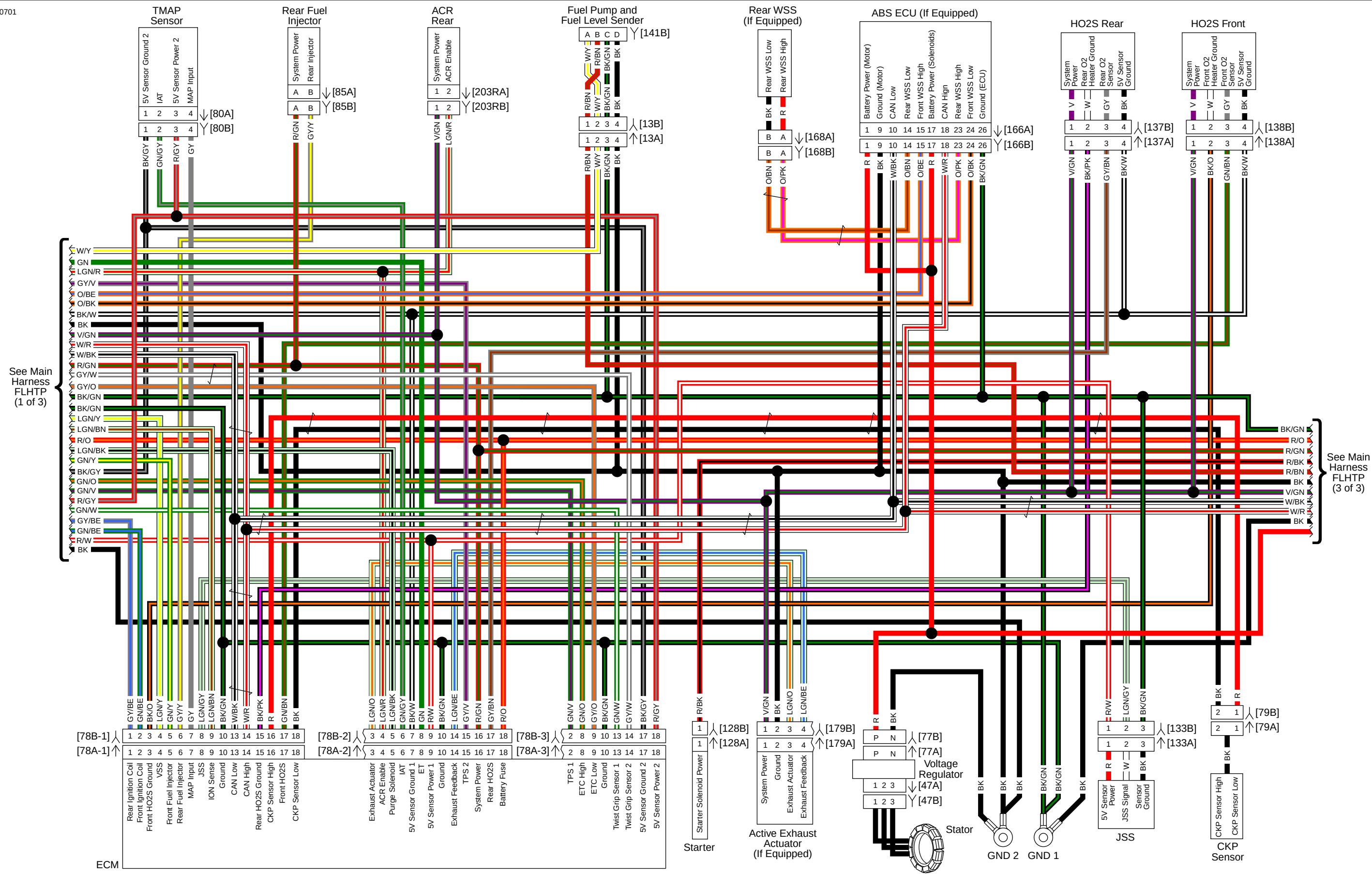
Main Harness (2 of 3): 2015 FLHTP
