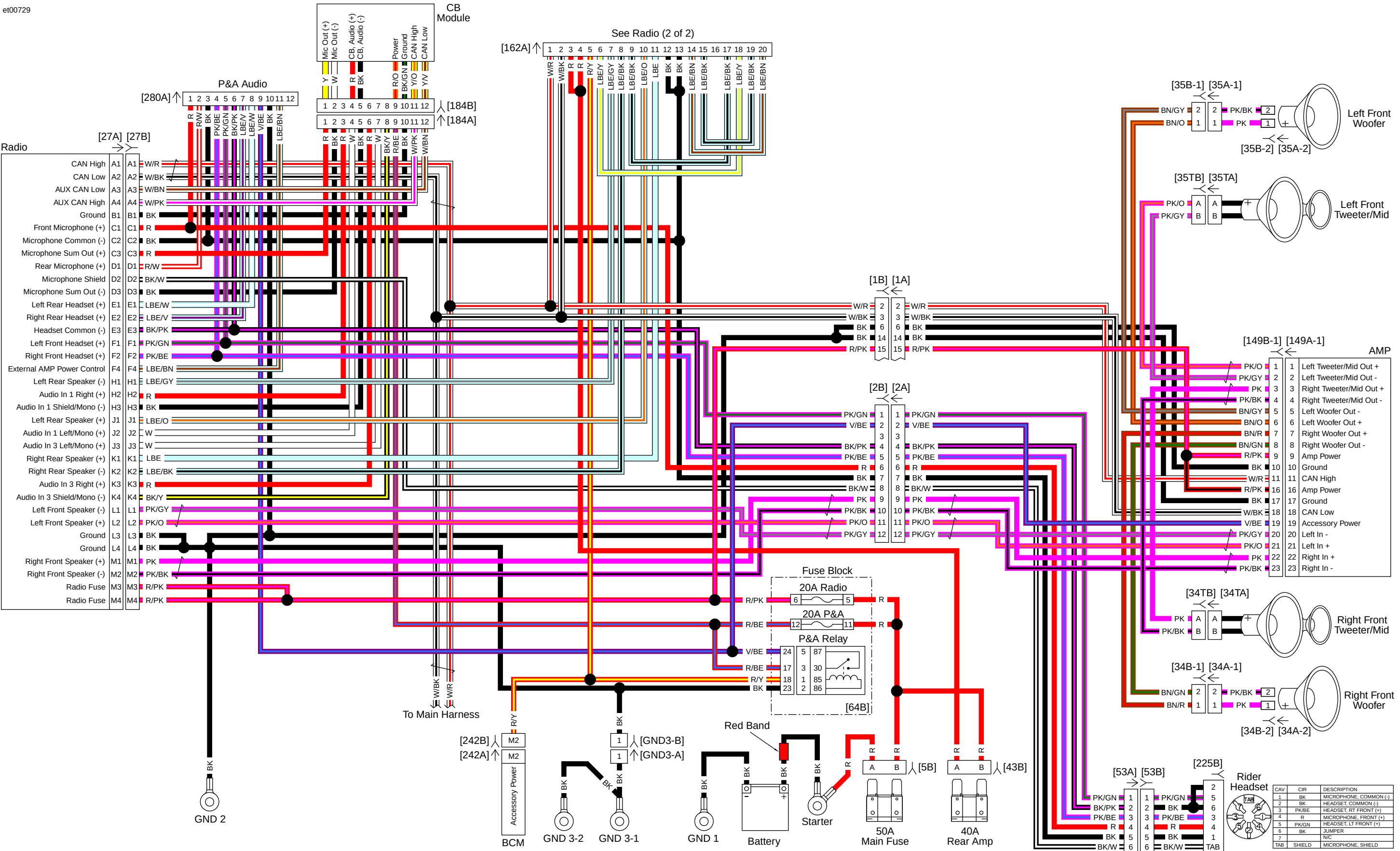
Radio (1 of 2): 2015 FLHXSE
