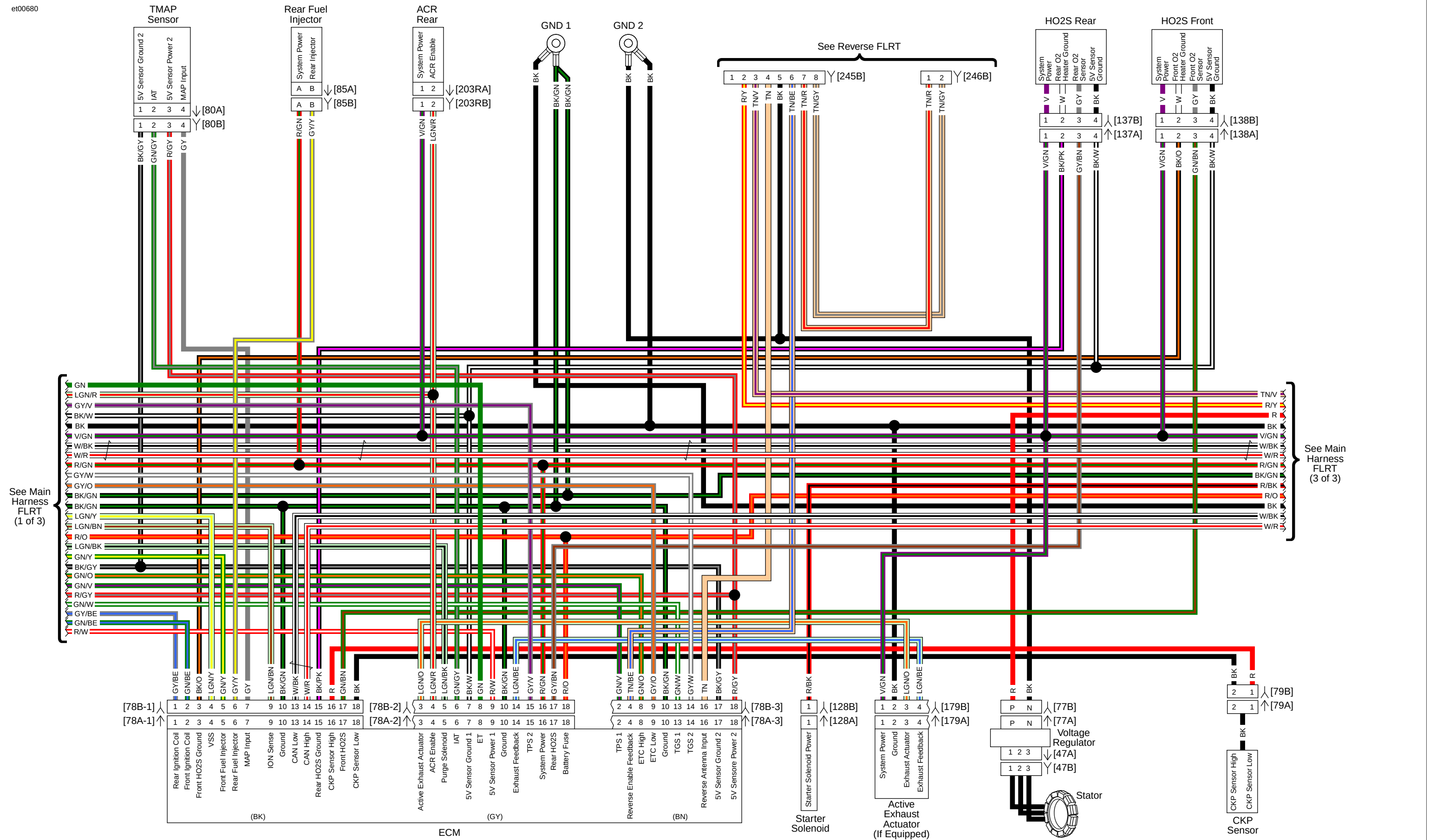
Main Harness FLRT (2 of 3): 2015 Trike Model
