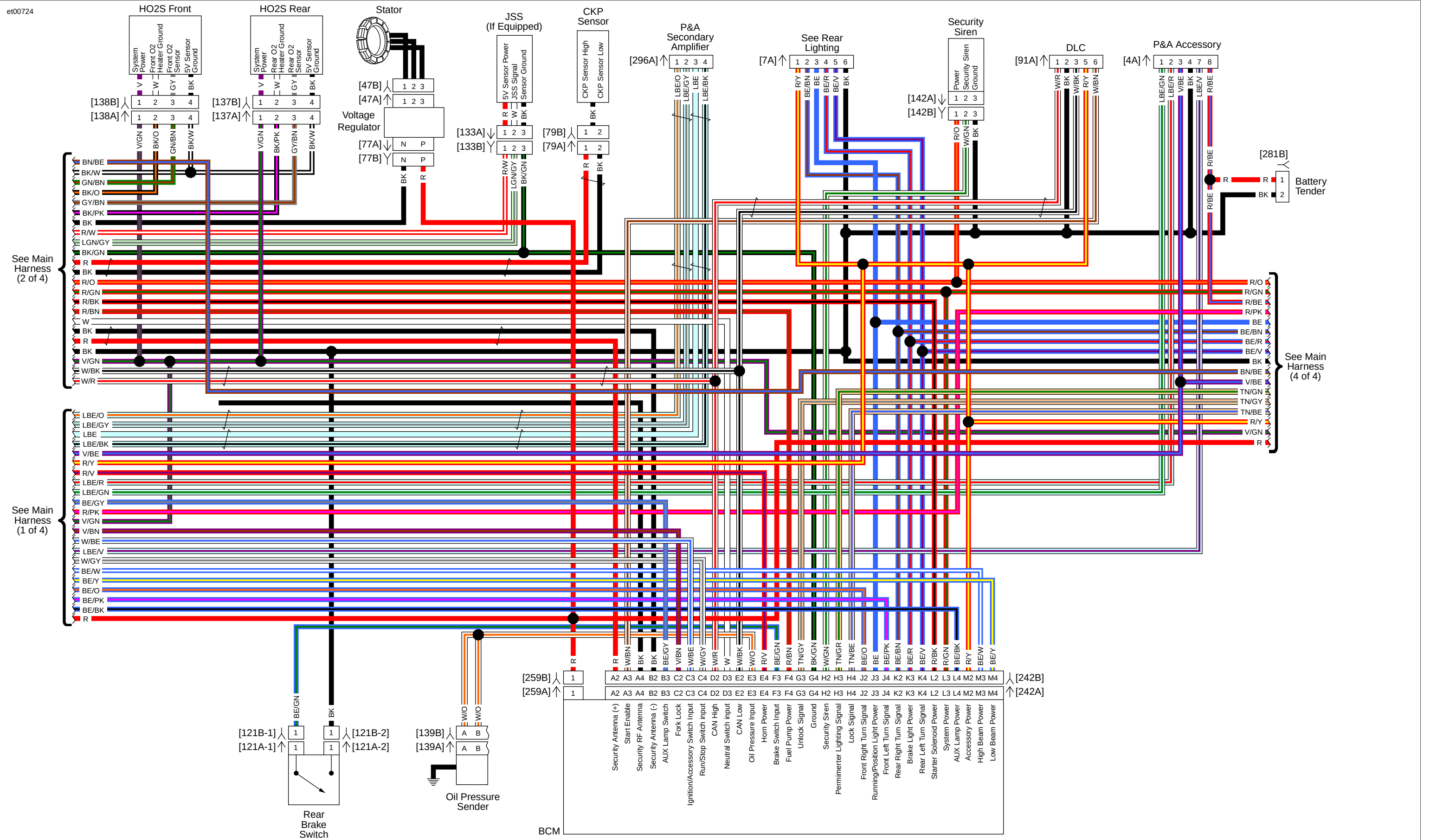
Main Harness (3 of 4): 2015 FLHTKSE
