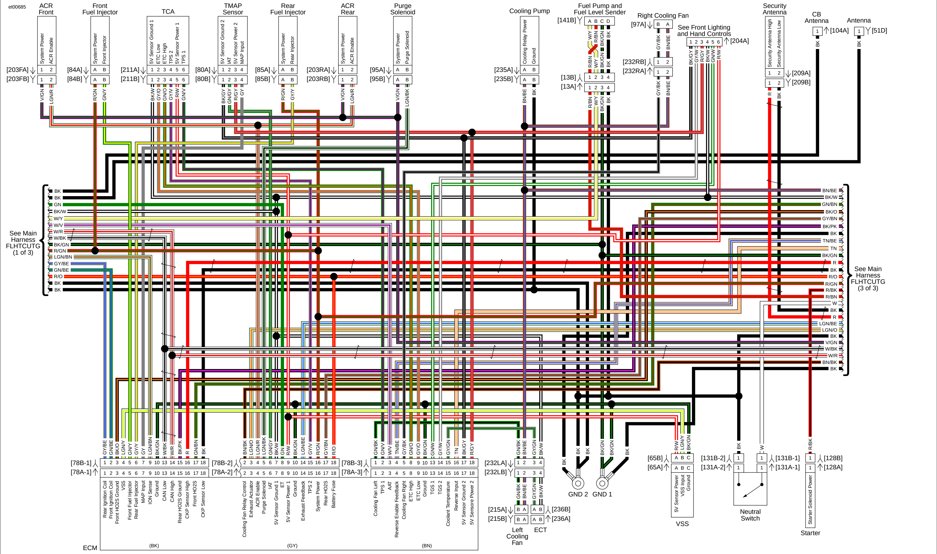
Main Harness FLHTCUTG (2 of 3): 2015 Trike Model
