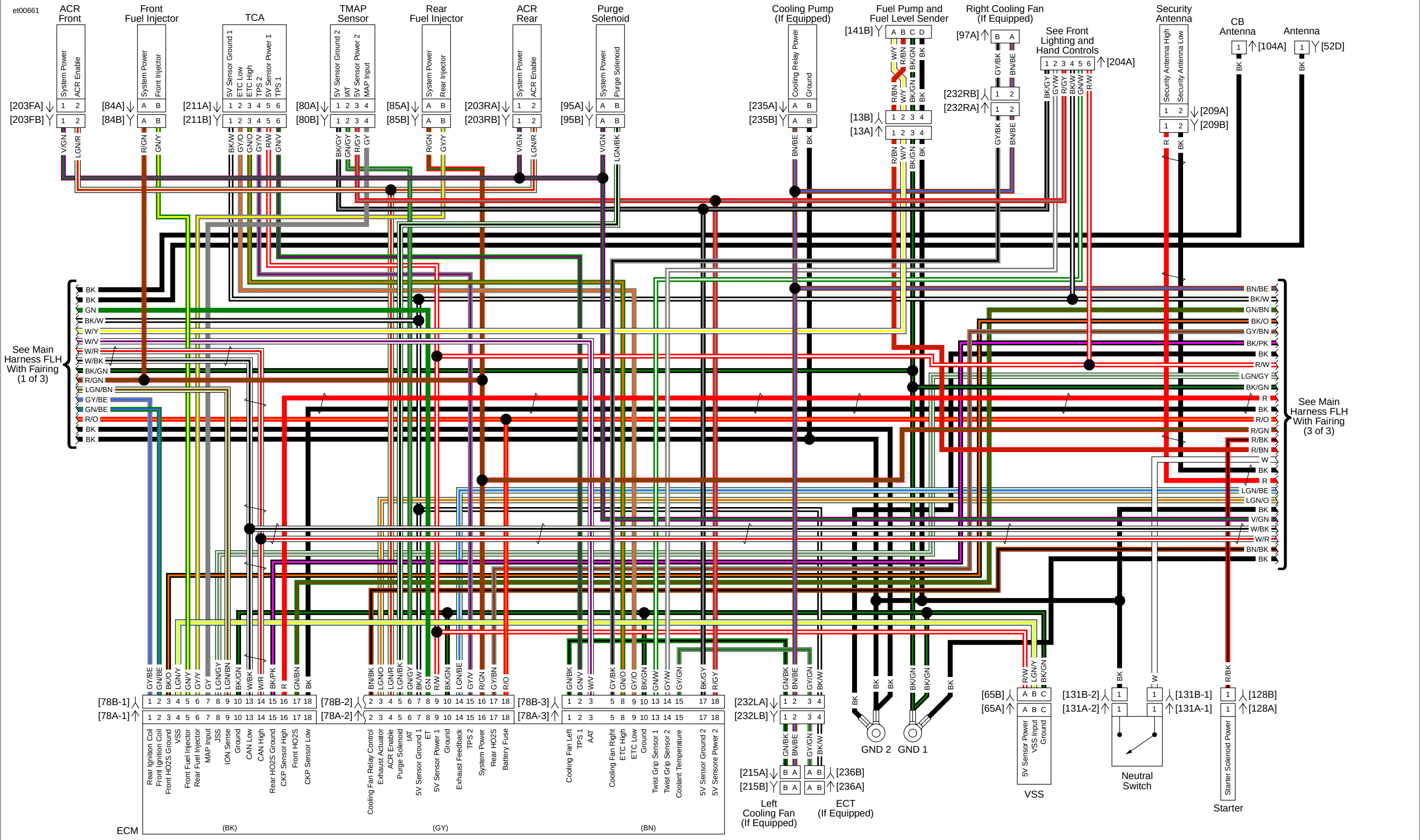
Main Harness FLH (2 of 3): 2015 Touring (With Fairing)
