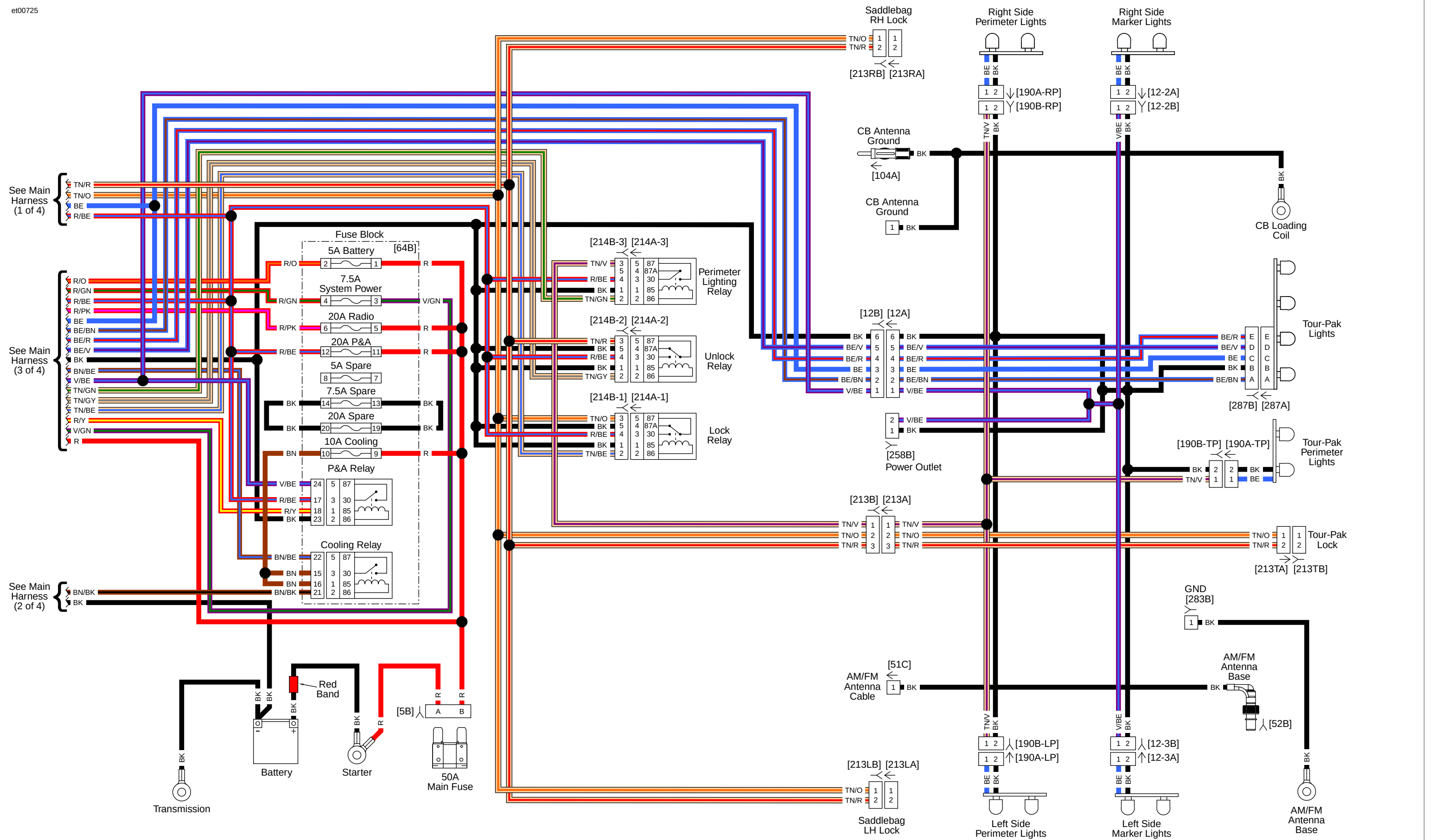
Main Harness (4 of 4): 2015 FLHTKSE
