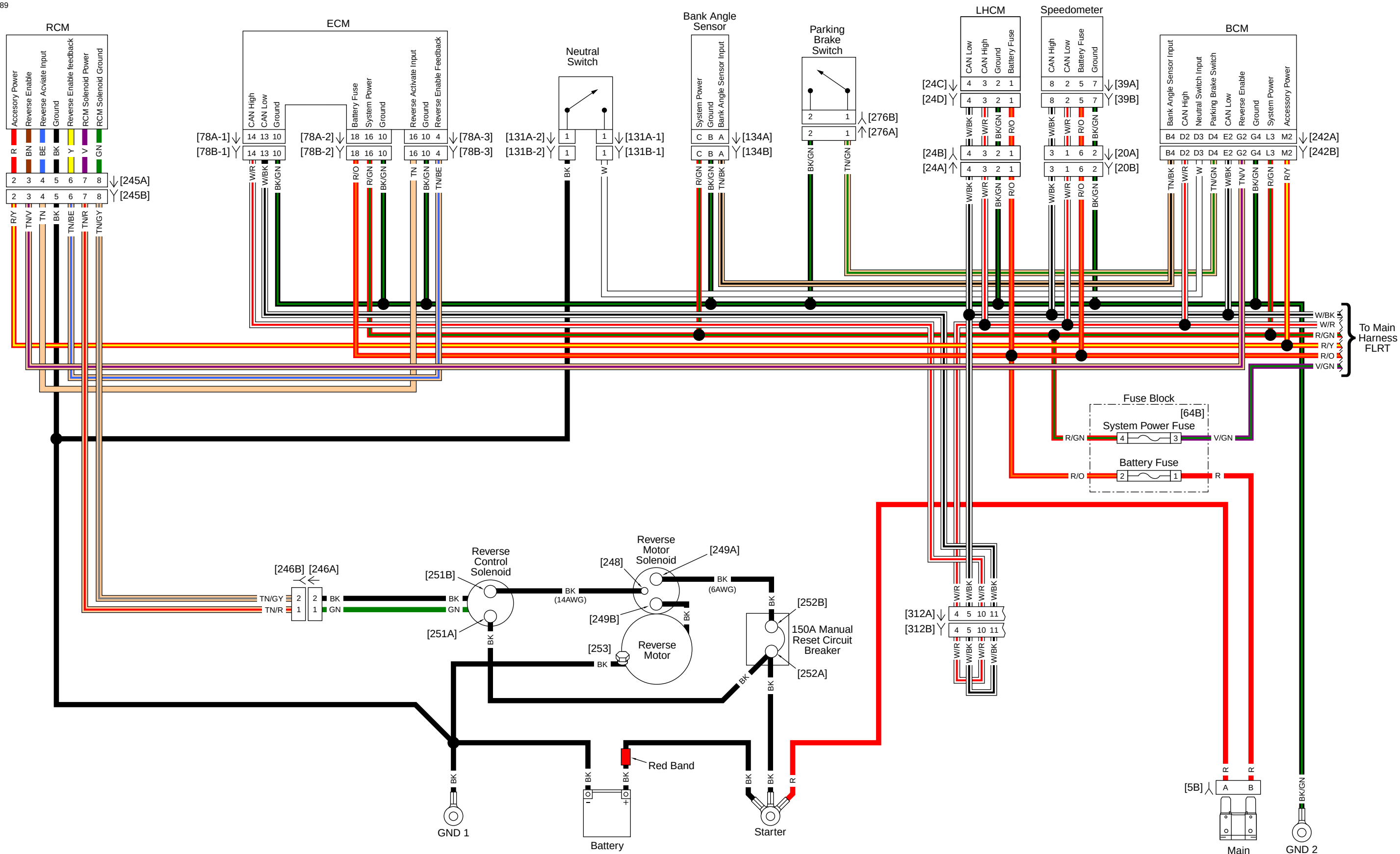
Reverse FLRT: 2015 Trike Model
