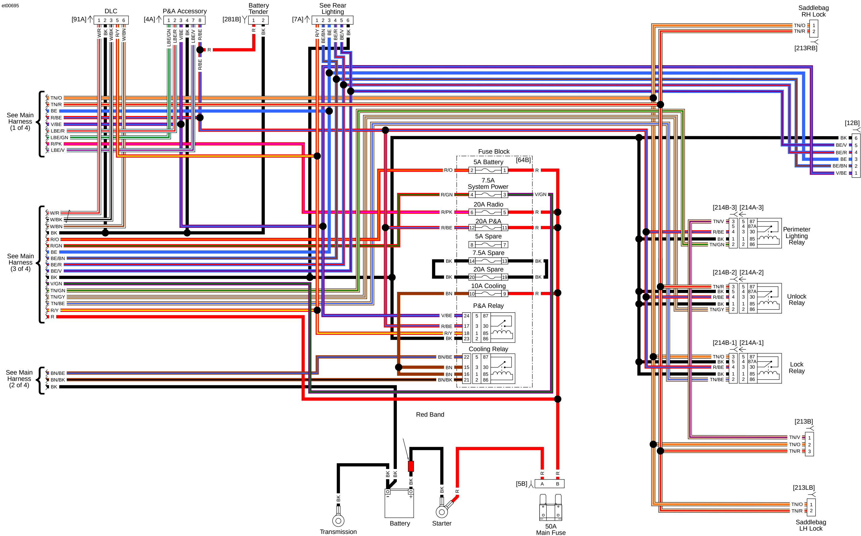
Main Harness (4 of 4): 2015 FLTRUSE
