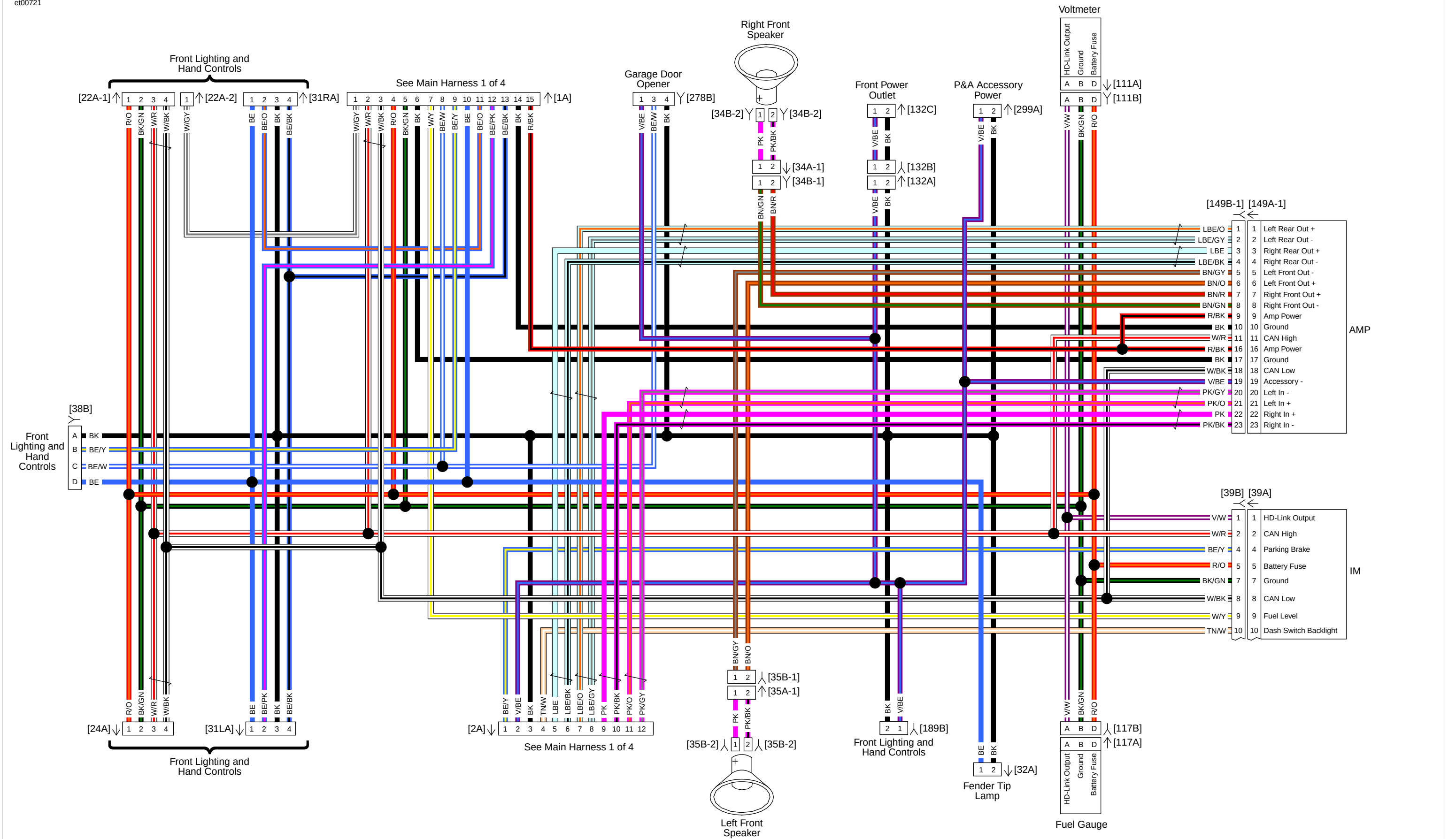
Fairing Harness: 2015 FLHTKSE
