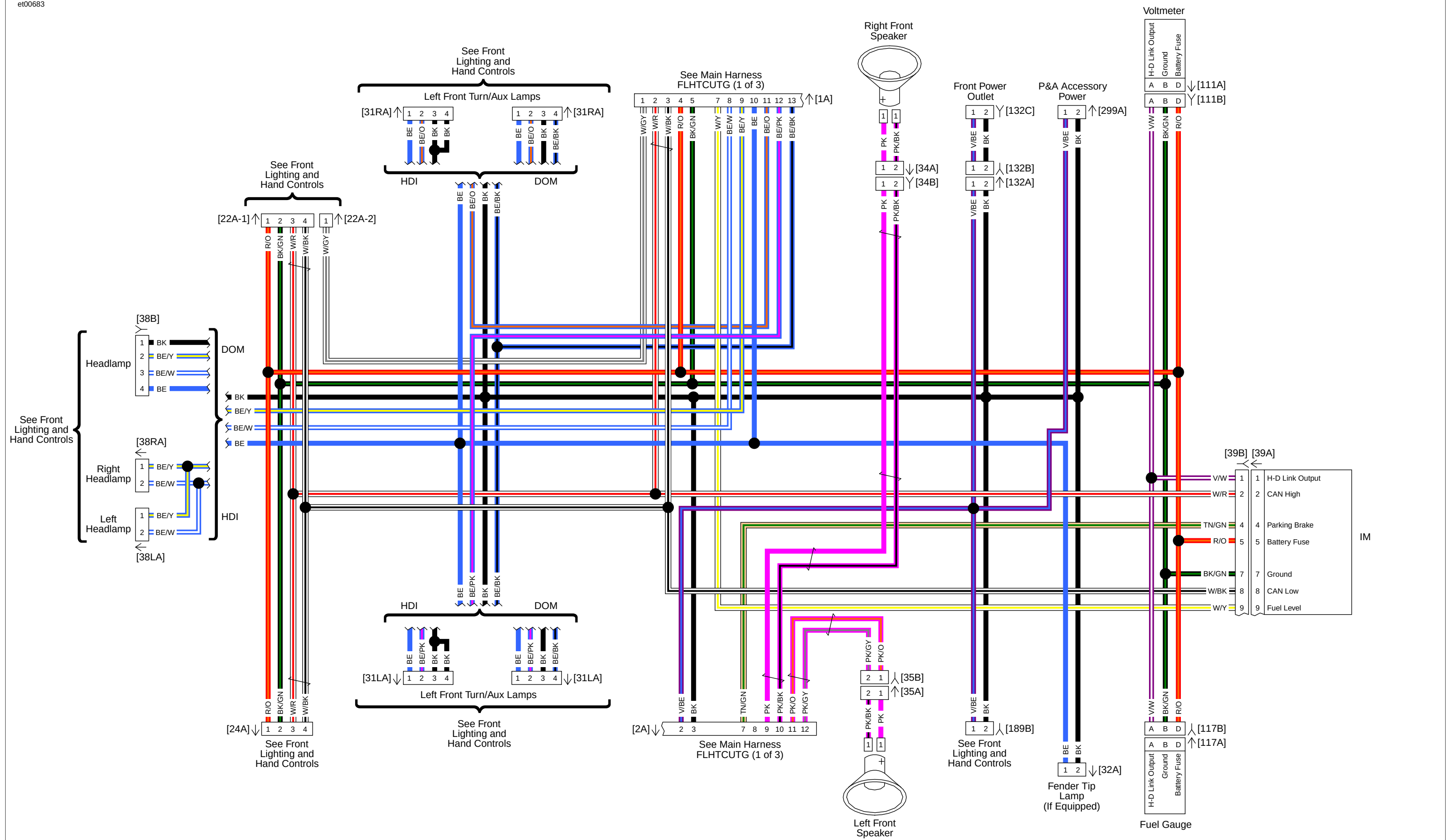
Fairing Harness FLHTCUTG: 2015 Trike Model
