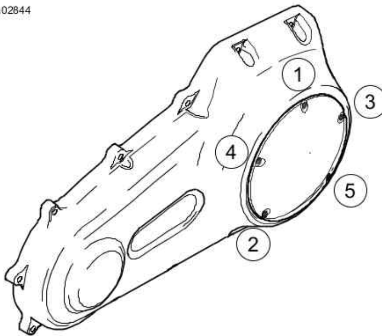
Clutch Cover Torque Sequence
